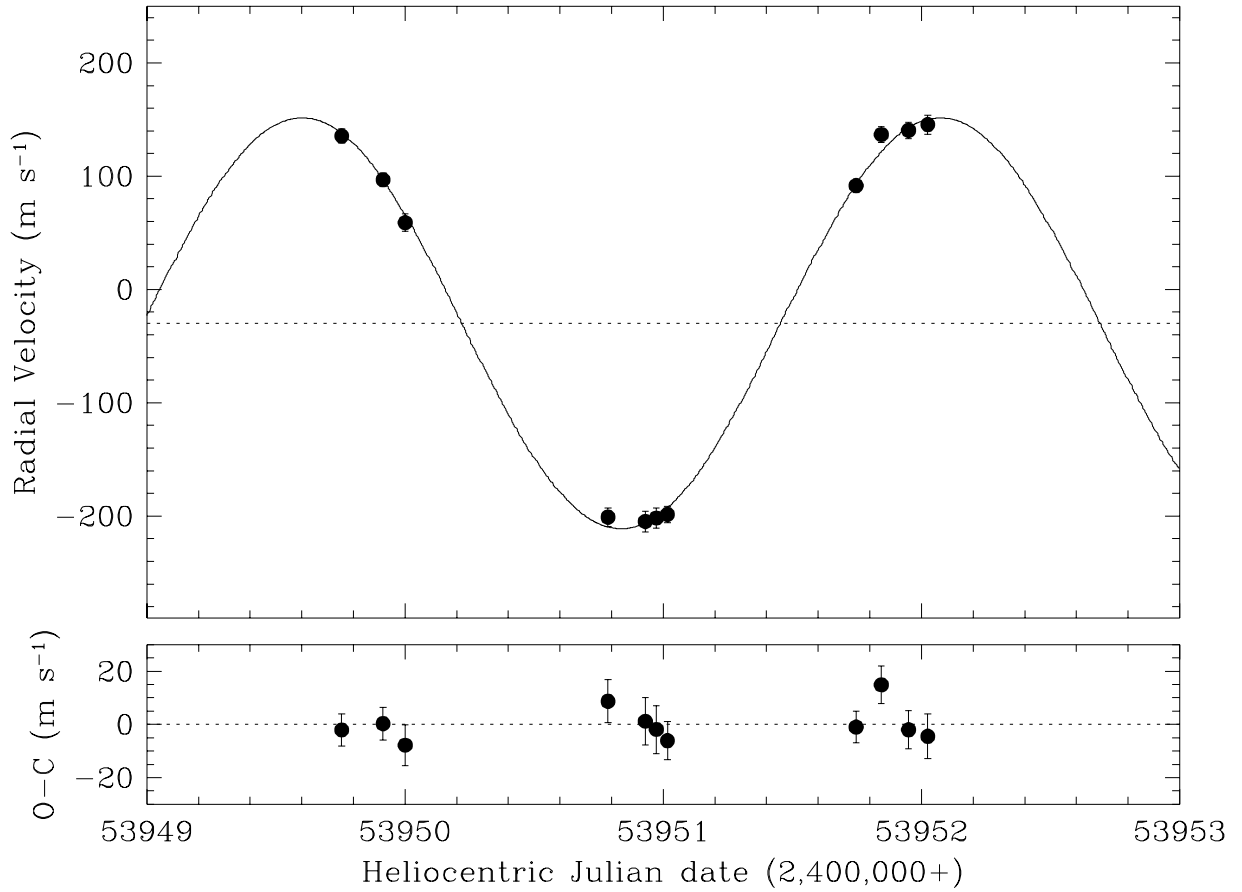
Fig. 2.— (Top panel) Radial-velocity observations of TrES-2 obtained with Keck/HIRES using the I 2 cell. The best-fit orbit ( solid line ) and \gamma -velocity ( dashed line ) are overplotted. (Bottom panel) The residuals from the best-fit model to the radial-velocity data.
