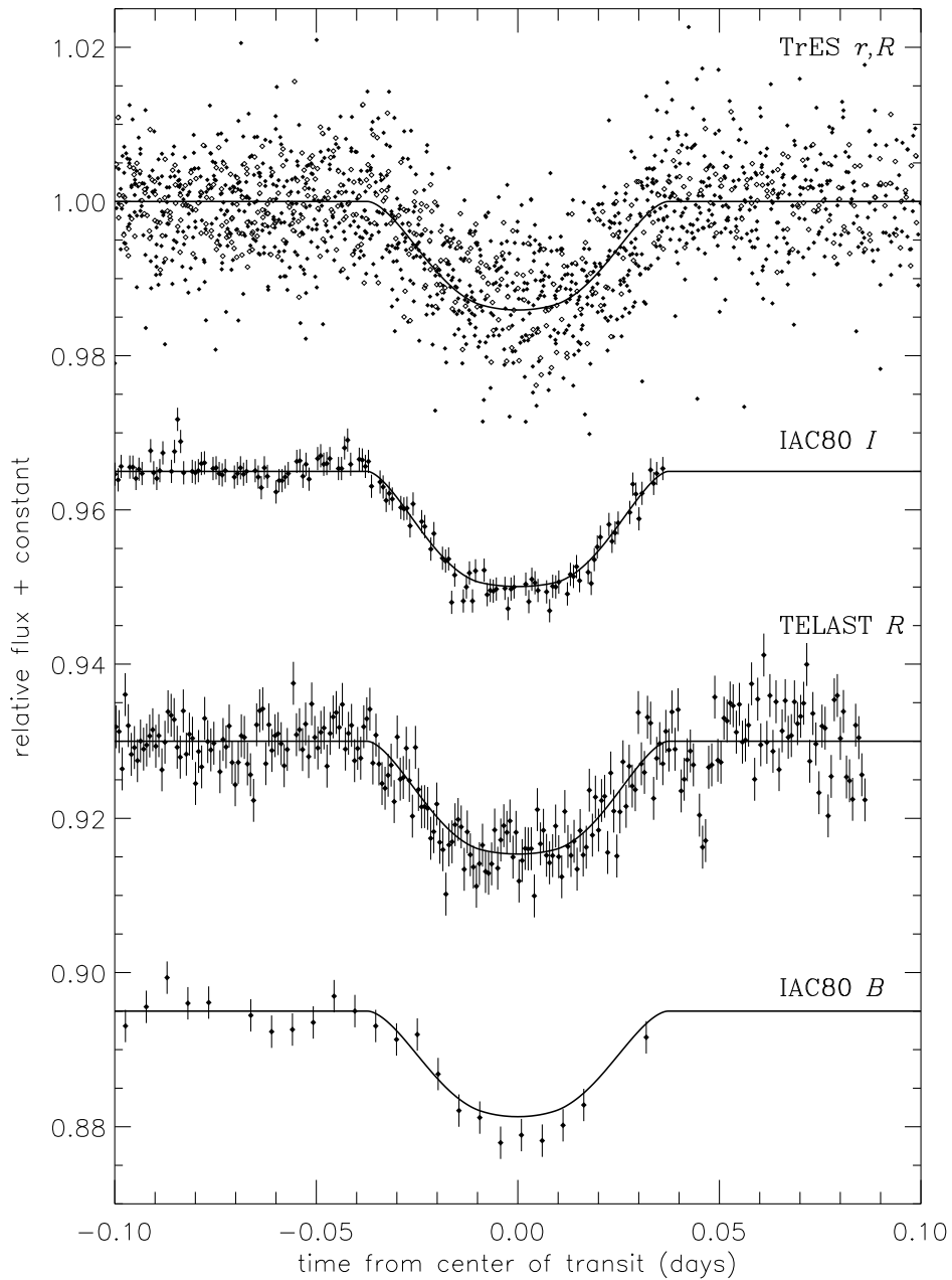
Fig. 1.— Relative flux of the TrES-2 system as a function of time from the center of transit, assuming the ephemeris in Table 2. The top light curve shows the unbinned discovery data, consisting of points from Sleuth r ( solid diamonds ) and PSST R ( open diamonds ). Each of the follow-up light curves is labeled with the telescope and filter employed. We have overplotted the simultaneous best-fit solution, assuming the appropriate quadratic limb-darkening parameters for each band pass.
