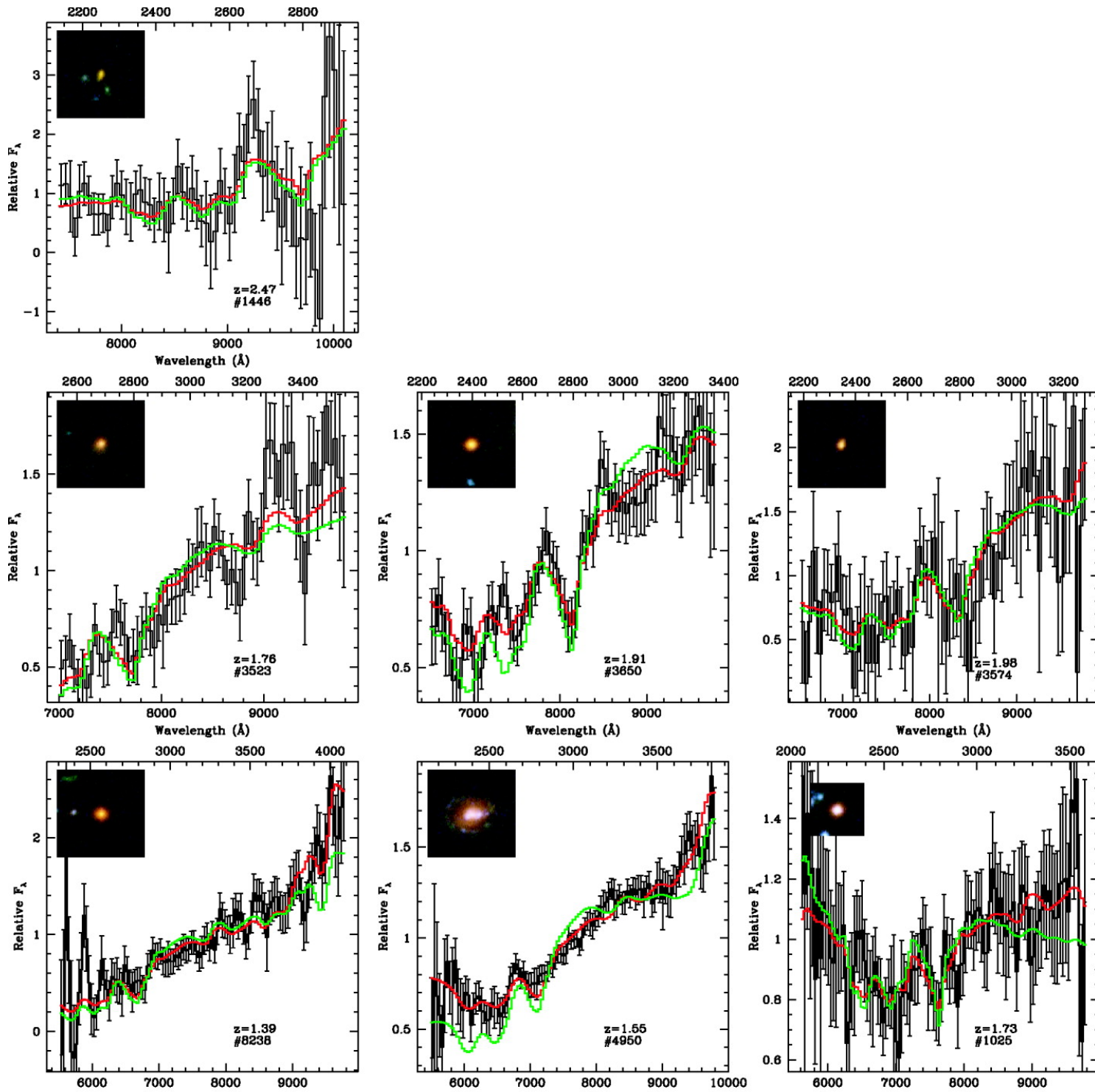
Figure 13: Spectra of galaxies with 1.4 < z < 2.5 in the Hubble Ultra Deep
