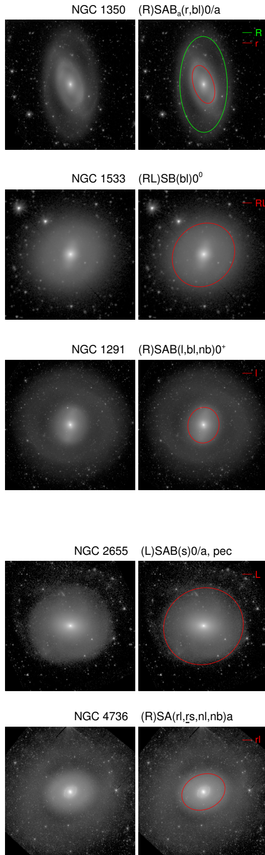
Fig. 1. Examples of the structure components identified in the classification by Buta et al. (2015). In each case one or more of the measured features are shown on top of the 3.6\ \mu\text{m} images from S 4 G.
