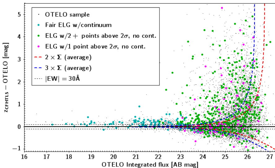
Figure 3: A colour-magnitude diagram for emission line object selection. OTELO integrated flux (OTELONB in text) corresponds to the flux measured on the deep image of the survey. Colour is defined using the z-band from CFHTLS and the OTELO data. Small black dots represent OTELO sources, and the large coloured ones are the bona-fide emitters (1031). Apart from the latter, additional 2253 sources show a colour > 3 \times \Sigma limit (upper blue segmented curve), which constitutes a parallel set of emission line objects that are being also analysed. The dotted black lines represent arbitrary colour boundaries of |EW| = 30 \text{ \AA} .
