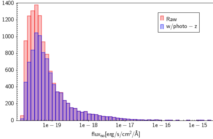
Figure 2: Histogram of the fluxes of the 11237 sources detected in OTELO survey. The minimum detectable flux at 3\sigma with 50% completeness is 2 \times 10^{-20} erg/cm 2 /s/Å, equivalent to 26.53 AB magnitudes, two magnitudes deeper than the deepest narrow band survey so far available. Light shadow corresponds to the whole sample of 11237 sources, while the darkest shadow represents the sample of more than 9000 sources with counterparts in the ancillary data.
