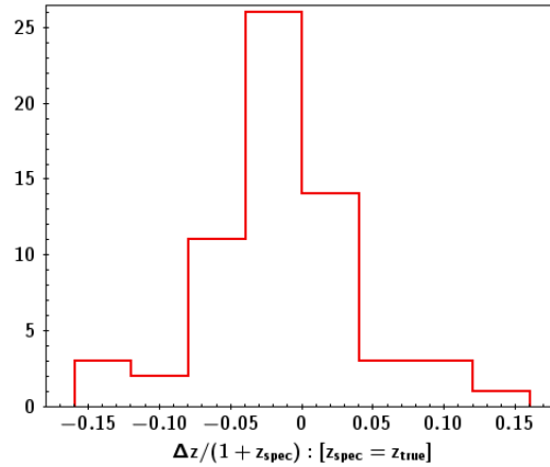
Figure 5: Photometric redshift errors for the emitters selected via pseudo-spectra.
