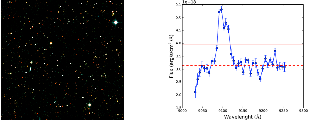
Figure 1: Left: Composite image of the OTELO field encompassing CFHTLS r & g bands plus OTELO deep image (OTELONB) obtained adding selected images together, as described in the text. North is at the top, East is at the left. Right: Pseudo-spectra of one z = 0.4 OTELO source showing the H\alpha plus [NII]\lambda 6583\text{\AA} emission lines. The dashed line is the continuum level and the solid line is 2\sigma above the continuum level.
