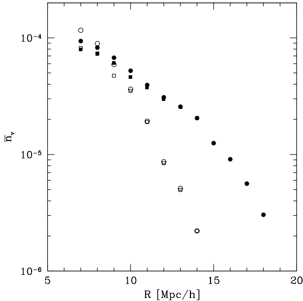
Figure 2. Number density of voids in numerical simulations obtained with our two void finders (squares for the CELLS void finder and circles for the HB void finder). These results were obtained using our 80h^{-1}\text{Mpc} and 120h^{-1}\text{Mpc} boxes. The open circles and squares denotes the number density of voids defined by halos with masses larger than 1 \times 10^{12}M_{\odot} while the filled circles and squares are the number density of voids defined by halos with masses larger than 5 \times 10^{12}M_{\odot} . Here, we can see that both algorithms get the same results as voids are bigger (symbols are overlapped). However, as we go to more common voids the differences between codes are bigger. This is due to the fact that the HB void finder is not so efficient detecting common voids (see text for details).
