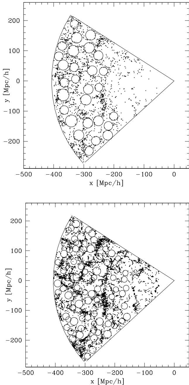
Figure 3. Voids in the 2dFGRS. We show the maximal spheres in the NGP1 volume-limited sample of galaxies (filled circles). The upper panel shows the voids with radius larger than 7.5h^{-1}\text{Mpc} defined by galaxies brighter than M_{b_j} = -20.5 - 5\log h . There are 2074 galaxies in this sample. In the lower panel we show the voids with radius larger than 13.0h^{-1}\text{Mpc} defined by galaxies brighter than M_{b_j} = -19.32 - 5\log h . The number of galaxies is 19695. Some galaxies lie inside the maximal spheres due to projection effects.
