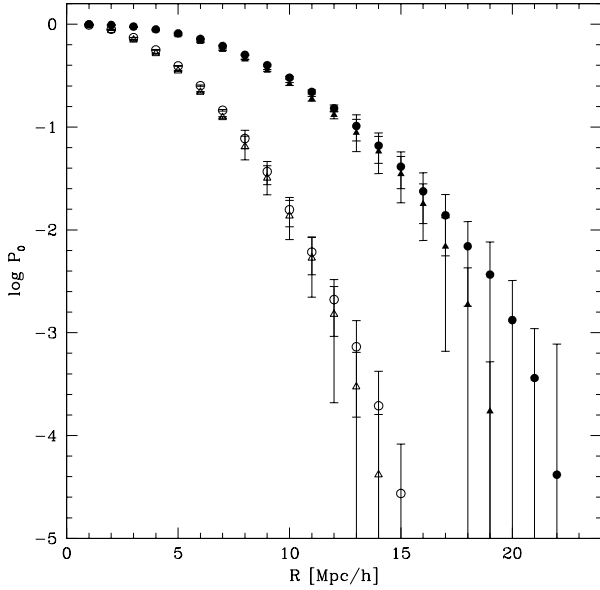
Figure 4. Void Probability Function for the 2dFGRS. We show the VPF for the SGP1,2 samples (open and filled circles respectively) and also for the NGP1,2 samples (filled and open triangles respectively).
