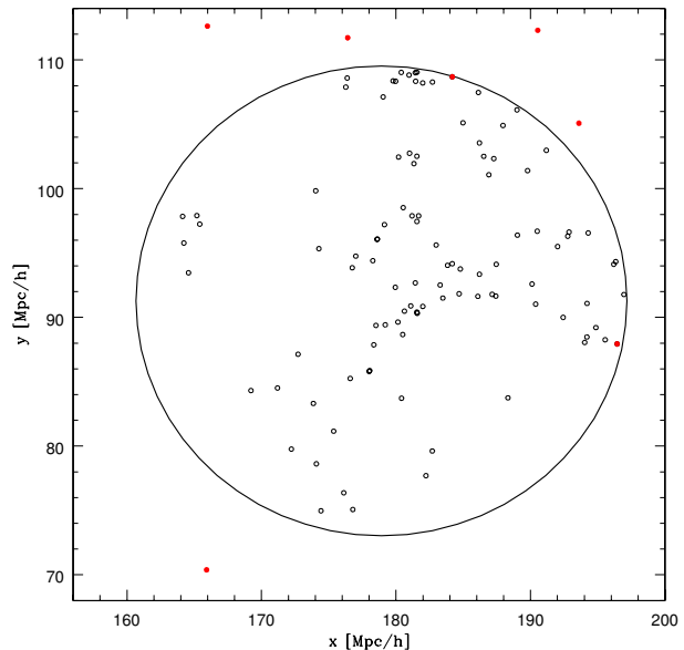
Figure 7. Galaxies inside a common void. We show a central 8h^{-1} \text{Mpc} thick slice of a 18.25h^{-1} \text{Mpc} void defined by galaxies brighter than -20.5 + 5 \log h (filled circles). The galaxies inside the void are fainter down to M_{b_j}^{\text{lim}} = -18.3 + 5 \log h (open circles).
