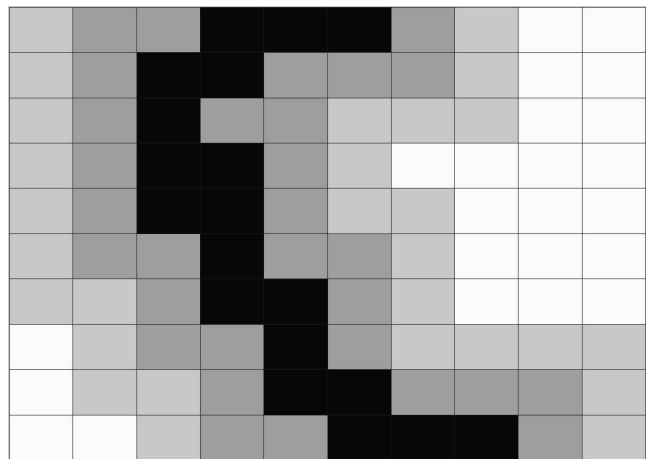
Figure A1. An example of labeling of cells for our Cell Void Finder . In order to save computational time, we mark the empty cells (dark grey cells) that are neighbours of those cells that contain objects (black cells). Note that this is an iterative process, i.e. we can now mark the empty cells that are neighbours of already marked empty cells (light grey cells). The stop of this iteration depends on the adopted resolution. The center of the void will be searched over the empty unmarked cells (white cells).
