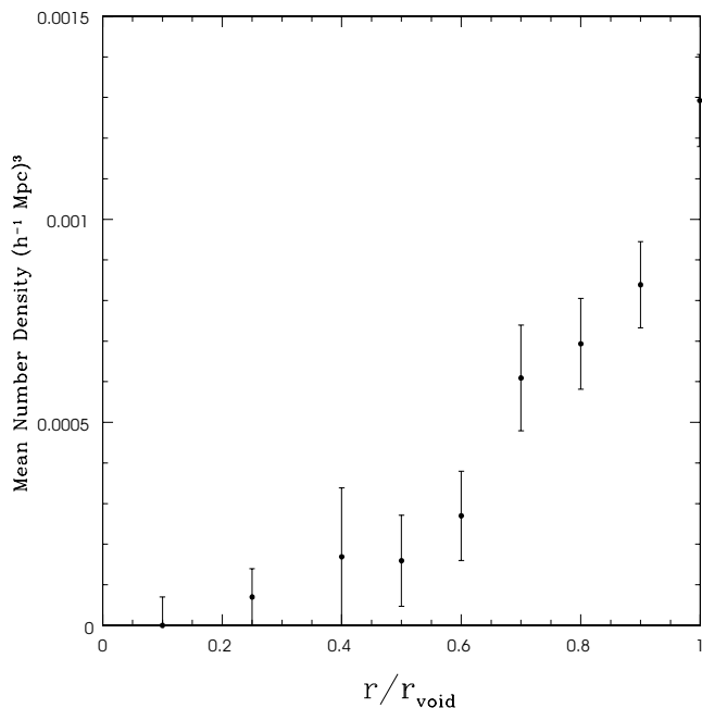
Figure 6. Averaged enclosed number density profile of faint galaxies ( -19.32 + 5 \log h < M_{b_j} < -18.3 + 5 \log h ) in nearby voids as a function of the distance from the center of the void (in void radius units). The mean number density of galaxies in the field for these magnitude band is 7.0 \times 10^{-3} (h^{-1} \text{Mpc})^{-3} .
