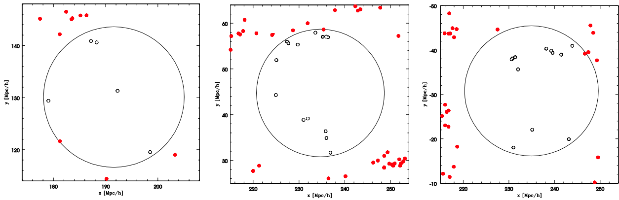
Figure 5. Three examples of faint galaxies in voids. We show for each void a 6h^{-1}\text{Mpc} central slab. In the left panel is shown a 13.5h^{-1}\text{Mpc} void, in the central panel a 14.0h^{-1}\text{Mpc} void and in the right panel a 14.7h^{-1}\text{Mpc} void. The filled circles are the galaxies brighter than -19.32+5\log h that define the voids. The open circles are the fainter galaxies inside the voids down to M_{b1}^{\text{lim}} = -18.3+5\log h . Note that even though there is not a large population of faint galaxies in these voids, the galaxies are not randomly distributed, i.e. they are distributed in filamentary structures similar to those found in another scales (see central and right panel).
