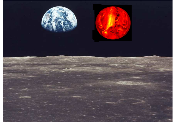
Fig. 1.— Earth views from the Moon. The picture illustrates a real image of the Earth, in the visible, taken by the Apollo 11 astronauts in 1969. Over-plotted is a global composite of the water vapor in the atmosphere, mapped in the IR range, by the GOES satellites. LTO would obtain continuous observations of the Earth both in the visible and infrared. Note that the two images correspond to different dates, seasons and geometries so the weather patterns do not correspond to each other, but are plotted for illustration only. In reality, the IR emission from the Earth as seen from the Moon, will be slightly brighter from the sunlit part of the Earth than from the night side.
