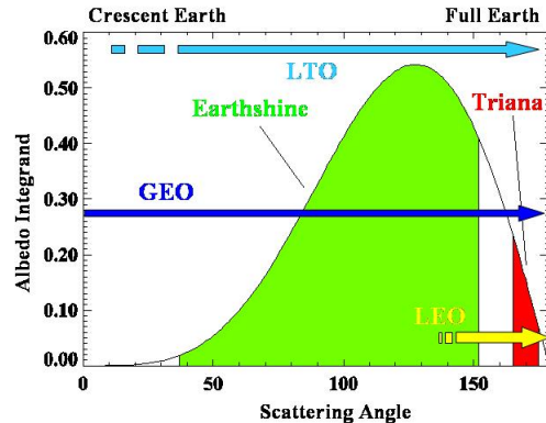
Fig. 2.— The kernel ( f_L(\theta) \sin(\theta) ) from which the Bond albedo is determined, shown as a function of observing angle. Its behavior is dominated by the Lambert phase function for small phase angles and by \sin(\theta) for large phase angles. The kernel coverage by the ground-based earthshine observations (green), a satellite orbiting about L1 assuming the proposed orbit of Triana (red), a satellite in LEO (yellow), a satellite in GEO (dark blue) and the proposed LTO (light blue), is shown. Adapted from Palte et al. (2003)
