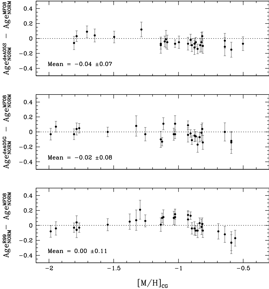
Fig. 9.— Comparison with previous works using the CG metallicity scale. The differences between the normalized ages of De Angeli et al. (2005) (using HST snapshot -deA05S- and ground based -deA05G- data) and Rosenberg et al. (1999) (R99) and the results derived in this paper by using D07 models (MF08) are indicated.
