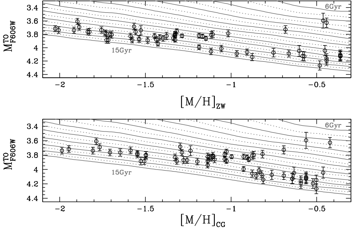
Fig. 5.— Theoretical TO absolute magnitudes from the D07 stellar evolution library. Lines represent M_{F606W}^{TO} for different ages as a function of global metallicity, in 1 Gyr (solid lines) and 0.5 Gyr (dashed lines) age steps. The lower isochrone corresponds to an age of 15 Gyr. Points represent the measured MSTO magnitudes. The upper panel shows the M_{F606W}^{TO} magnitude as a function of the metallicity in the ZW scale; the lower panel gives M_{F606W}^{TO} as a function of the metallicity in the CG scale.
