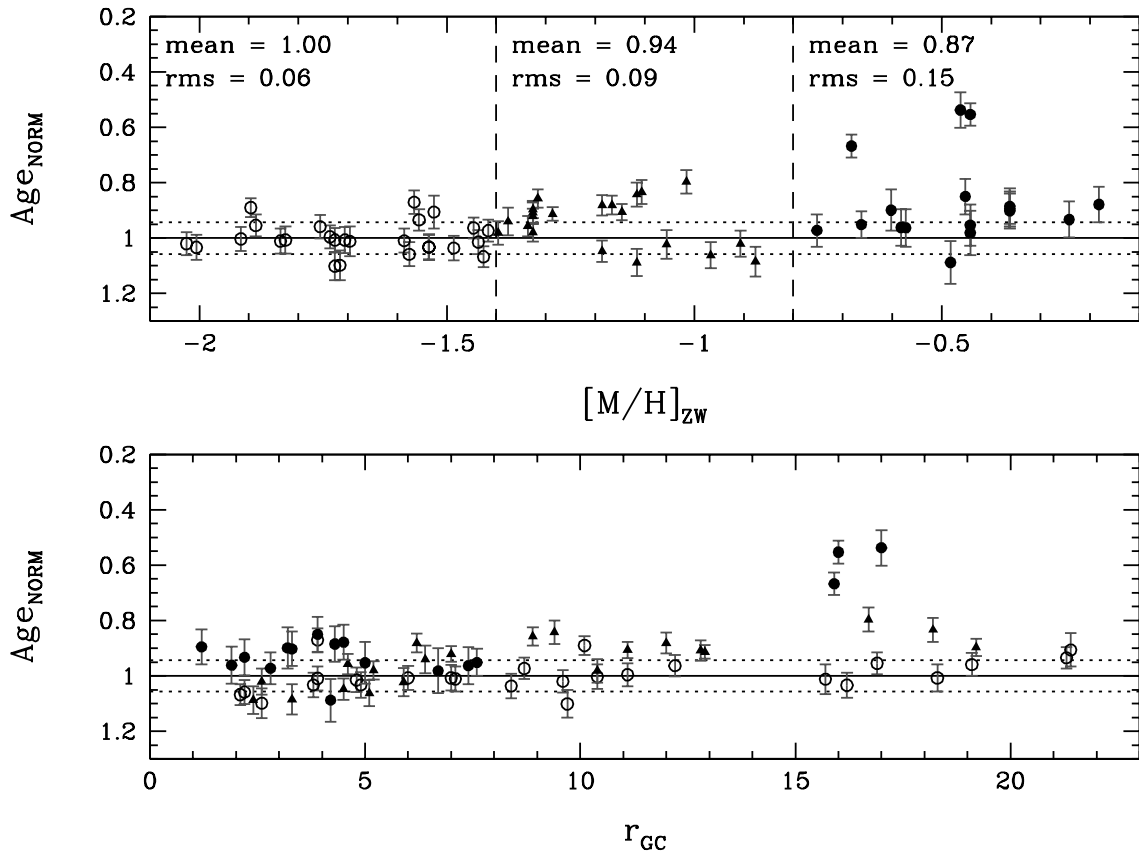
Fig. 11.— Same as Figure 10, but for the ZW metallicity scale.
