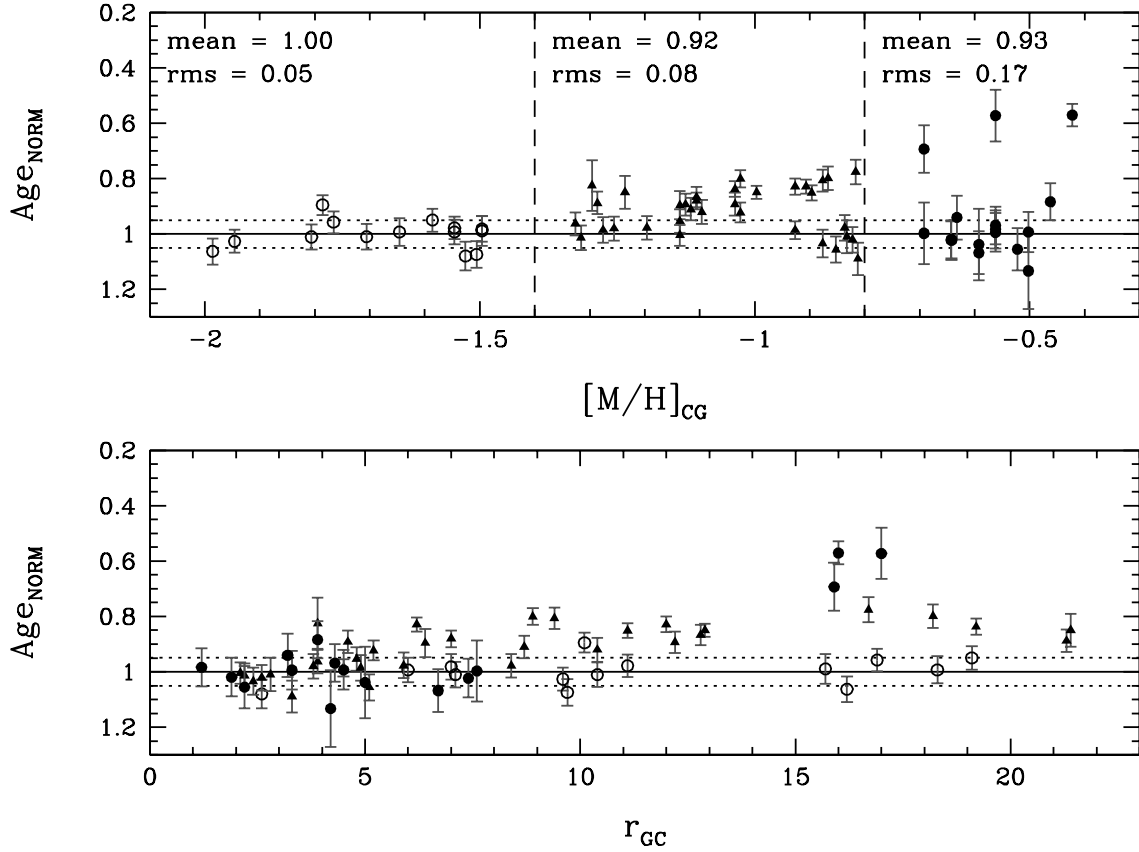
Fig. 10.— Globular cluster normalized ages as a function of [M/H] in the CG metallicity scale (upper panel), and as a function of galactocentric distance ( r_{GC} kpc, lower panel). These results have been derived using the D07 stellar evolution library. Open circles, filled triangles and filled circles represent GCs within the low–, intermediate– and high–metallicity groups, respectively. For each of the three metallicity groups, mean age and rms is indicated. See text for details.
