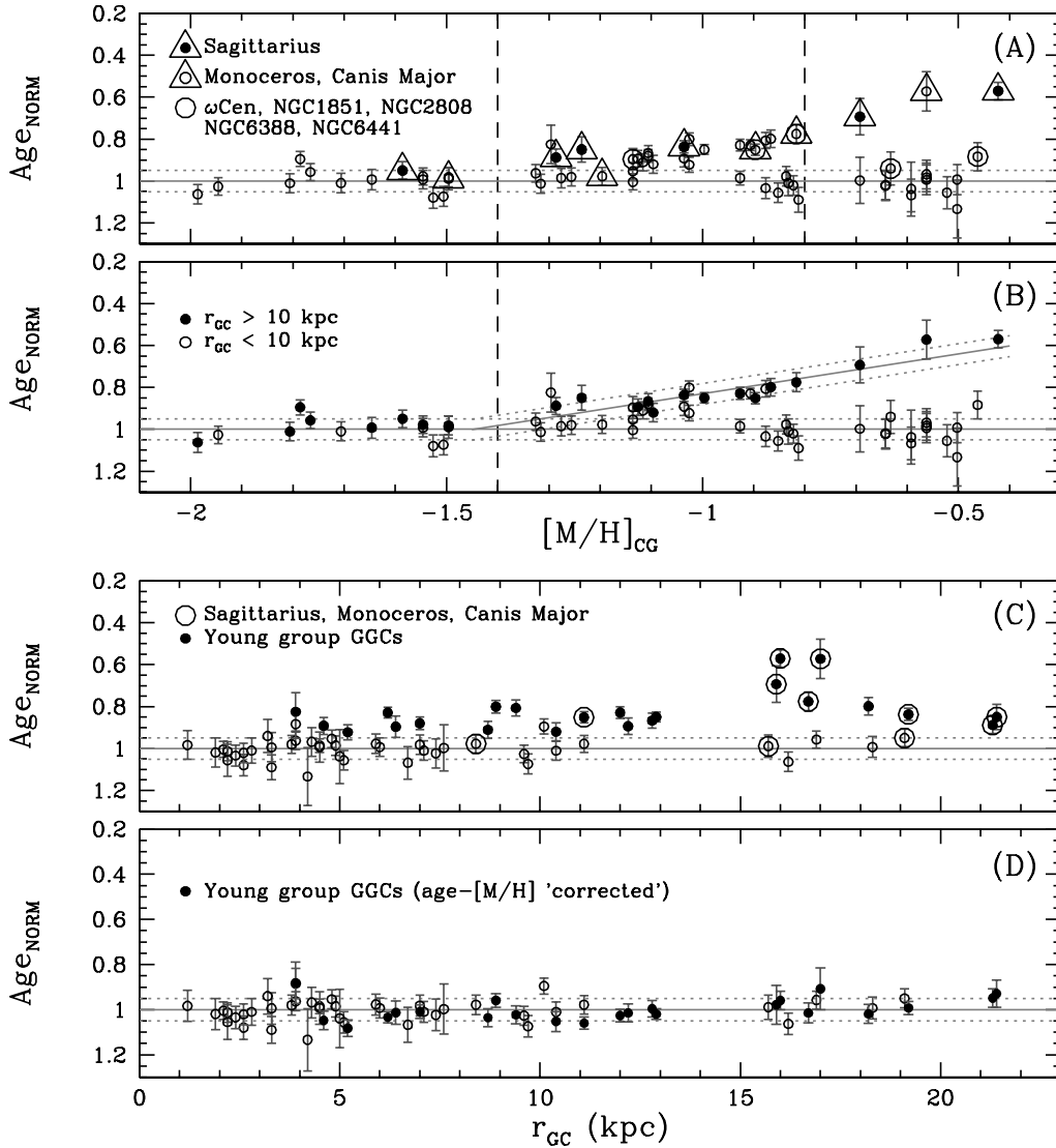
Fig. 13.— Age–metallicity relation using the CG metallicity scale (A and B) and normalized ages versus galactocentric distance (C and D). In A, clusters associated with Sagittarius, Monoceros and Canis Major have been marked, together with multiple stellar population clusters. In B, GGCs with r_{GC} < 10 kpc are represented with open circles, while those with r_{GC} > 10 kpc are plotted with filled circles. A least squares fit to the young group’s age–metallicity relation is also plotted. In C, Sagittarius, Monoceros and Canis Major’ clusters are also marked. Finally, D shows the same as C, but here ages of clusters in the young group have been age–metallicity ‘corrected’ using the age–metallicity relation shown in B. See text for details.
