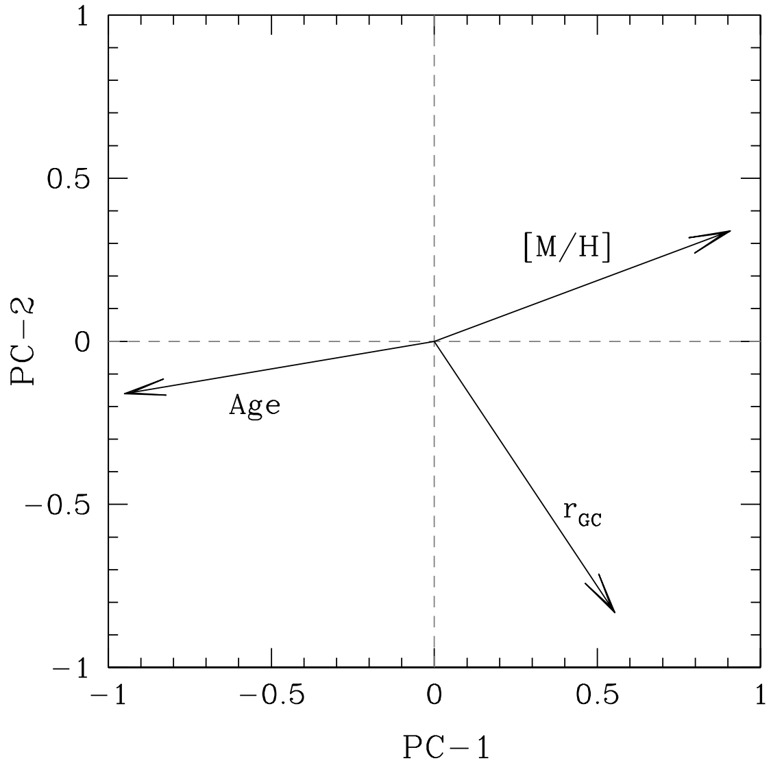
Fig. 14.— Young group principal–component (PC) analysis: Relations between original data and principal components on the first two principal components plane. It can be seen that the first PC is strongly correlated with [M/H] and age, but weakly with r_{GC} , while the second PC carries on most of the r_{GC} variance. See text for details.
