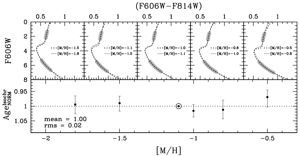
Fig. 6.— Testing the used main sequence fitting procedure and relative ages determination using 13 Gyr synthetic isochrones. Upper panel shows the MS–fitting for 13 Gyr synthetic isochrones with the same metallicities as the adopted reference clusters ( [M/H] = -0.5, -0.8, -1.0, -1.1, -1.5 and -1.8 ). Lower panel shows the obtained relative ages. The MSTO magnitude of the [M/H]=-1.1 isochrone (encircled point) has been considered as MSTO zeropoint.
