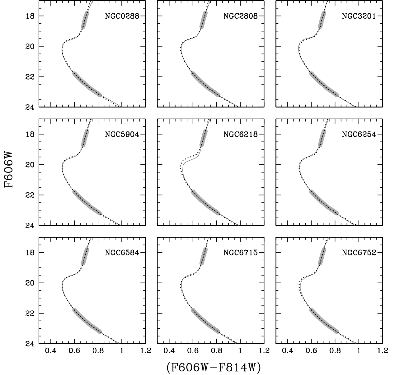
Fig. 3.— Examples of MS-fitting for the -1.3 \leq [Fe/H]_{CG} < -1.1 metallicity group. The reference cluster is NGC 6981 (dashed line). Each cluster MRL (solid line) has been fitted to the reference cluster in the magnitude intervals [(M_{F606W}^{TO} - 2.5) < M_{F606W} < (M_{F606W}^{TO} - 1.5)] and [(M_{F606W}^{TO} + 1.5) < M_{F606W} < (M_{F606W}^{TO} + 3.0)] (shaded regions).
