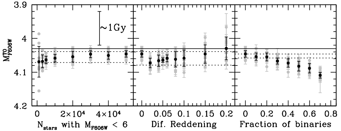
Fig. 4.— The right panel shows M_{F606W}^{TO} measurements over synthetic CMDs with 50,000 stars brighter than M_{F606W} = 6 , no differential reddening, and varying the fraction of binary stars. Grey points show the MSTO measurements for the 10 different CMDs generated in each case, and black points show the average and standard deviation of each of the 10 measurement sets. Solid line represents the MSTO’s magnitude measured directly on the isochrone. The Central panel shows the same as left panel, but now the fraction of binary stars is 0.0 and the maximum differential reddening is varying between 0.0 and 0.2. The left panel shows the same, but now the fraction of binary stars is 0.0, the differential reddening is 0.0 and the number of stars brighter then M_{F606W} = 6 is varying between 1,000 to 50,000. Dashed lines represent the adopted \pm\sigma in each case. See text for details.
