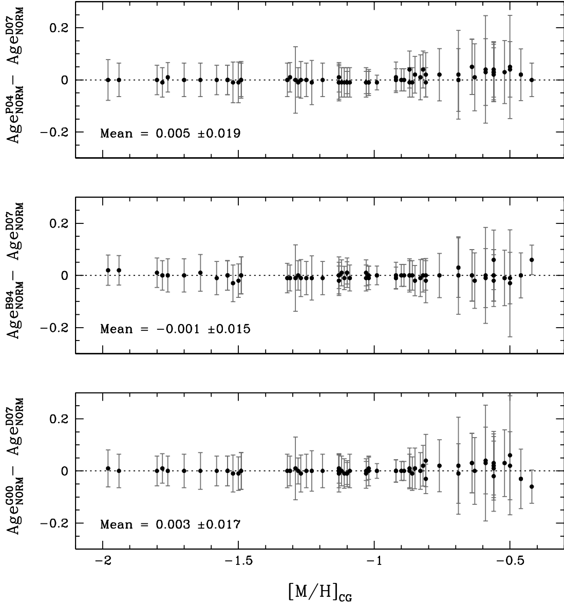
Fig. 8.— Comparison of normalized ages derived from different sets of models in the CG metallicity scale. The difference between normalized ages derived using P04, B94 and G00 models, respectively, and the D07 models are shown. It can be seen that relative ages derived using the main sequence fitting method are independent from the adopted model.
