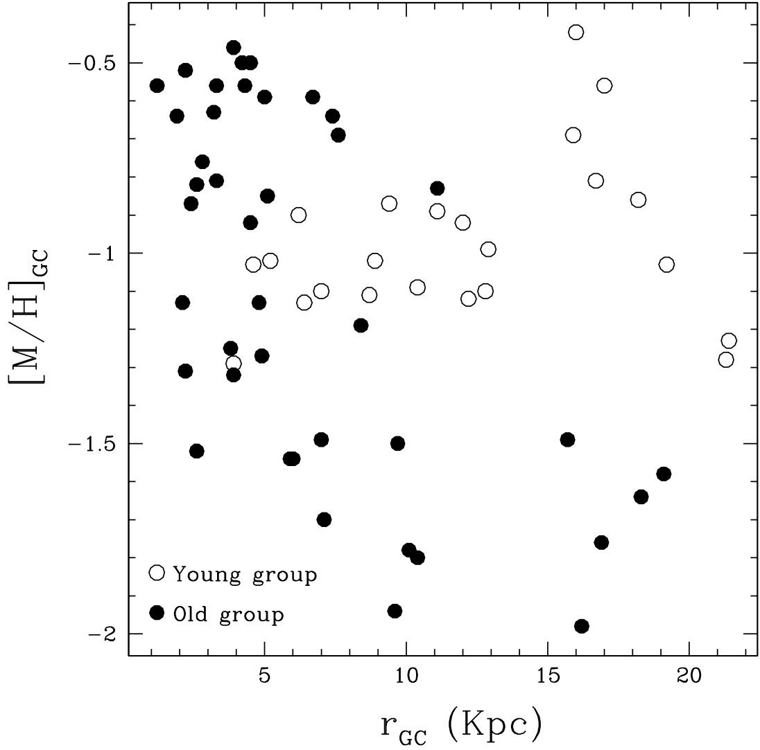
Fig. 12.— Globular cluster’s [M/H] in the CG metallicity scale as a function of the galactocentric distance. Open and filled circles represent clusters in the young and old groups, respectively.
