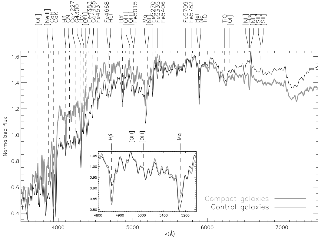
FIG. 2.— Average mean spectra of the compact galaxies of our sample (grey thick line) and the control galaxies (thin line). The individual spectra were previously convolved to the highest dynamical velocity dispersion ( 320 \text{ km s}^{-1} ) and divided by their corresponding means, so they contribute with the same weight. Each mean spectrum has been normalized by its mean flux within the spectral range showed in each panel. The inset shows the spectral regions around H\beta and Mg lines.
