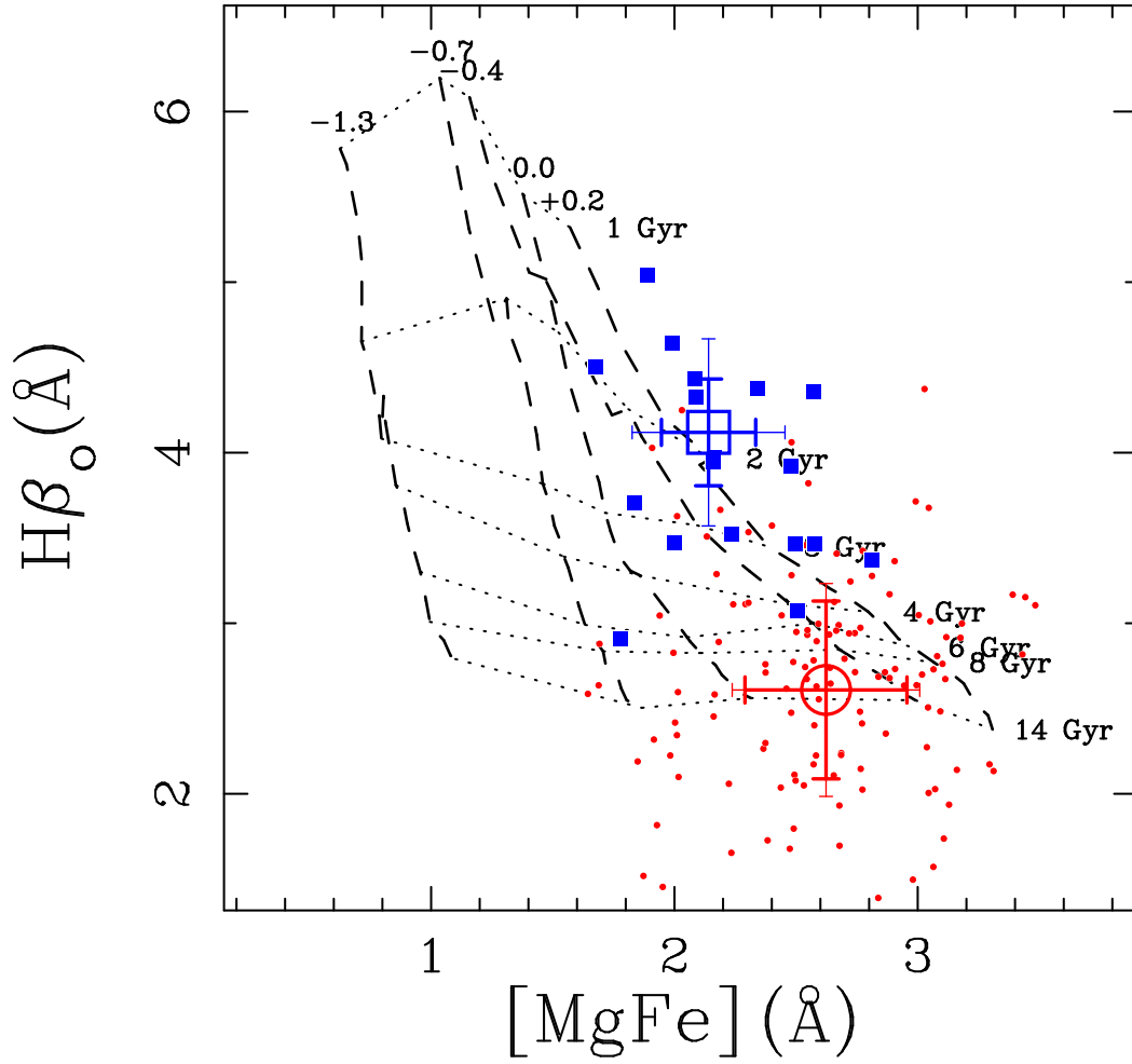
FIG. 3.— H_{\beta_0} vs [\text{MgFe}] diagram for 151 galaxies of the compact (filled squares, 18) and control samples (dots, 133) for which no \lambda 5577 \text{ \AA} [O I] skyline residuals affect the index measurements. Overplotted are V99+ SSP model grids with different ages (dotted lines) and metallicities (dashed lines) as given in the labels. The open square and circle are error-weighted mean indices for the compact and control samples respectively. Thick error bars show the 1\sigma index uncertainties, whereas the thin error bars correspond to the dispersions of the samples.
