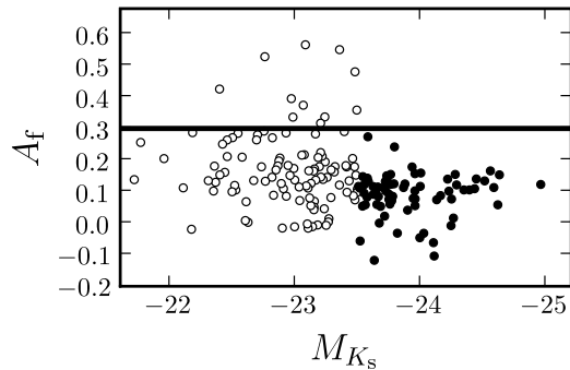
FIG. 5.— Asymmetry in function of M_{K_s} for blue ( white dots ) and red ( black dots ) samples (see the text for details). The black solid line shows the merger criterion A_{\text{m}} = 0.30 .
