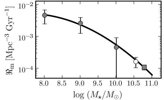
FIG. 7.— Major merger rate in function of stellar mass at z = 0.6 . The data are from Conselice et al. (2008, gray dots ), Bell et al. (2006, gray square , error bars are smaller than the symbol size), and this work ( white dot ). The solid line is the best equation (17) fit to the data.
