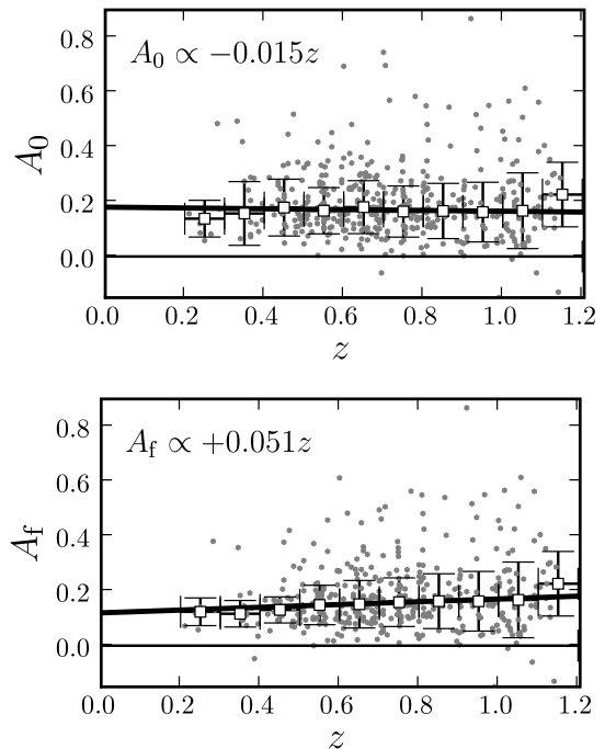
FIG. 4.— Asymmetry vs. redshift in the M_B \leq -20 sample ( gray dots in both panels). Upper : asymmetries of the sources measured on the original images. Lower : asymmetries of the sources measured on images degraded to z_d = 0.75 . White squares in both panels are the mean asymmetries in 0.1 redshift bins. The black solid line is the linear fit to the mean asymmetries in the [0.5, 0.8) redshift interval.
