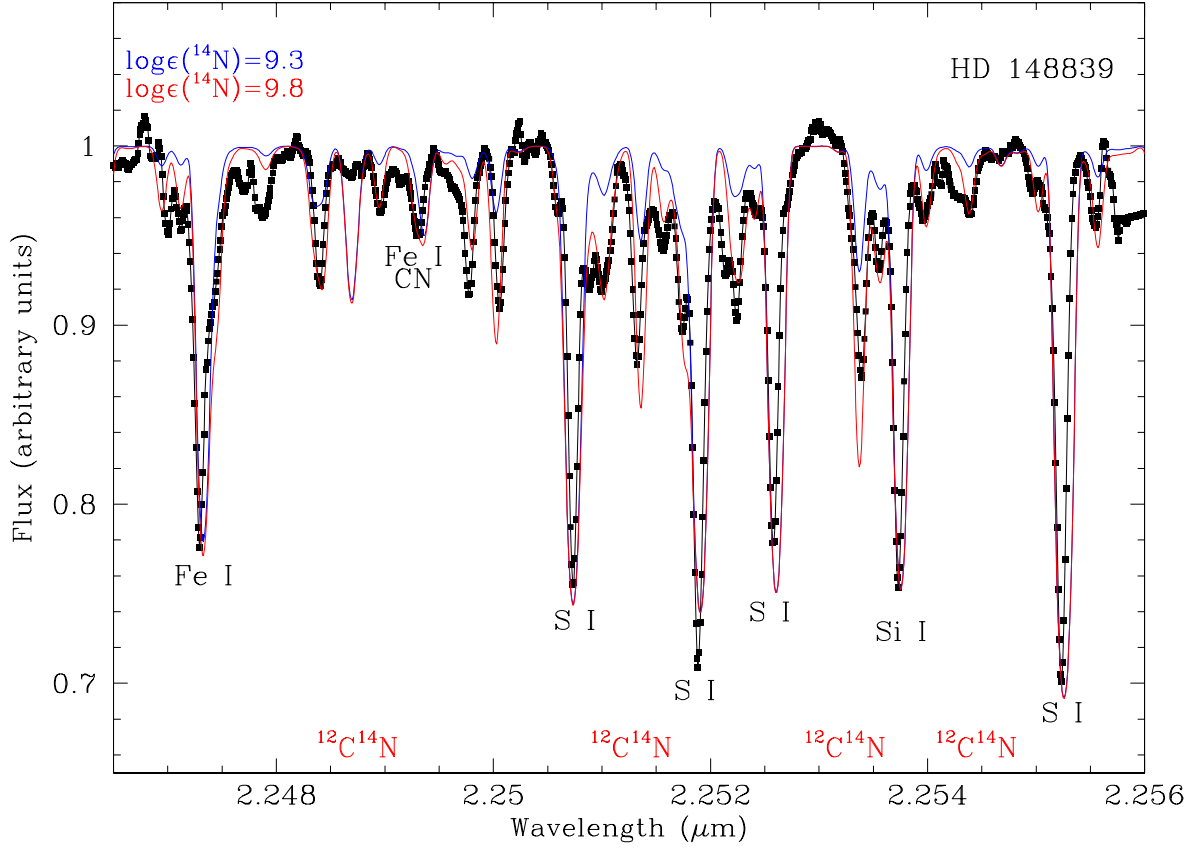
Fig. 19.— Best synthetic (red) and observed (black) spectrum for the CN region centered at \sim 2.251 \mu\text{m} for the HdC star HD 148839. The synthetic spectrum has been created assuming the input C abundance of 9.52, the N is in the form of ^{14}\text{N} with an abundance \log \epsilon(\text{N}) = 9.8 dex, and a total O abundance of \log \epsilon(\text{O}) = 9.2 . A synthetic spectrum (blue) for a lower ^{14}\text{N} abundance of \log \epsilon(\text{N}) = 9.3 dex is also shown for comparison.
