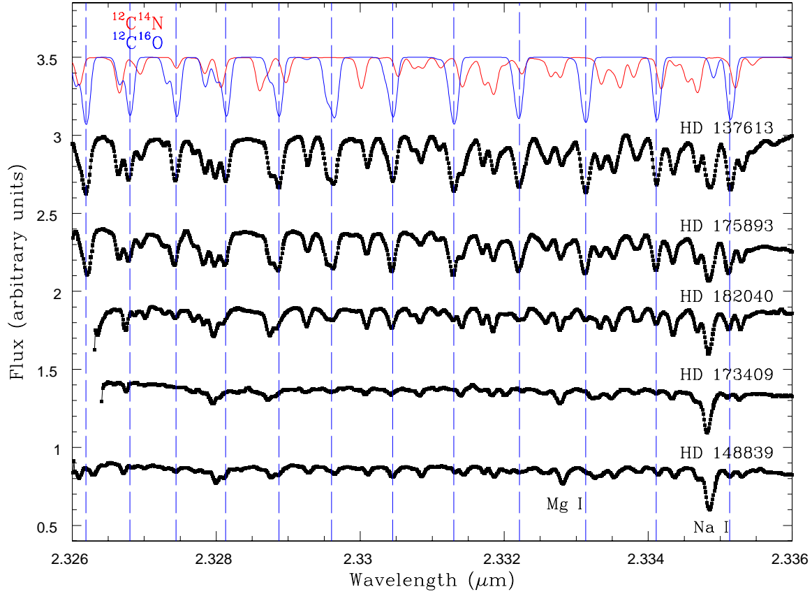
Fig. 3.— PHOENIX spectra centered at 2.331 \mu\text{m} for the five HdC stars. This region is dominated by lines of the ^{12}\text{C}^{16}\text{O} and ^{12}\text{C}^{14}\text{N} molecules but note the Na I line at 2.3348 \mu\text{m} . The strongest ^{12}\text{C}^{16}\text{O} lines are marked with a dashed blue vertical line. Synthetic spectra composed for HD 137613 for the CO and CN isomers ( ^{12}\text{C}^{16}\text{O} in blue and ^{12}\text{C}^{14}\text{N} in red) shown at the top indicate that these molecules dominate the spectra.
