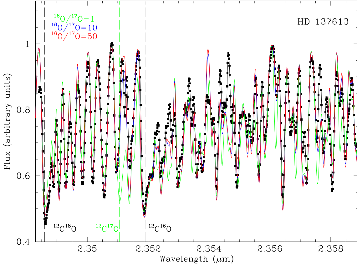
Fig. 14.— Best synthetic (red) and observed (black) spectrum in the region around the 2-0 2.349\mu\text{m} ^{12}\text{C}^{18}\text{O} bandhead for the ^{18}\text{O} -rich HdC star HD 137613. The red spectrum assumes the input C abundance of 9.52, the N abundance of 9.4, a total O ( ^{16}\text{O} + ^{17}\text{O} + ^{18}\text{O} ) of \log\varepsilon(\text{O})=8.7 and the isotopic ratios ^{16}\text{O}/^{18}\text{O}=0.5 and ^{16}\text{O}/^{17}\text{O}=50 . Synthetic spectra for lower ^{16}\text{O}/^{17}\text{O} ratios (or higher ^{17}\text{O} abundances) of 1 (green) and 10 (blue) but the same total O ( ^{16}\text{O} + ^{17}\text{O} + ^{18}\text{O} ) of \log\varepsilon(\text{O})=8.7 are shown for comparison. See Figure 11 for additional information.
