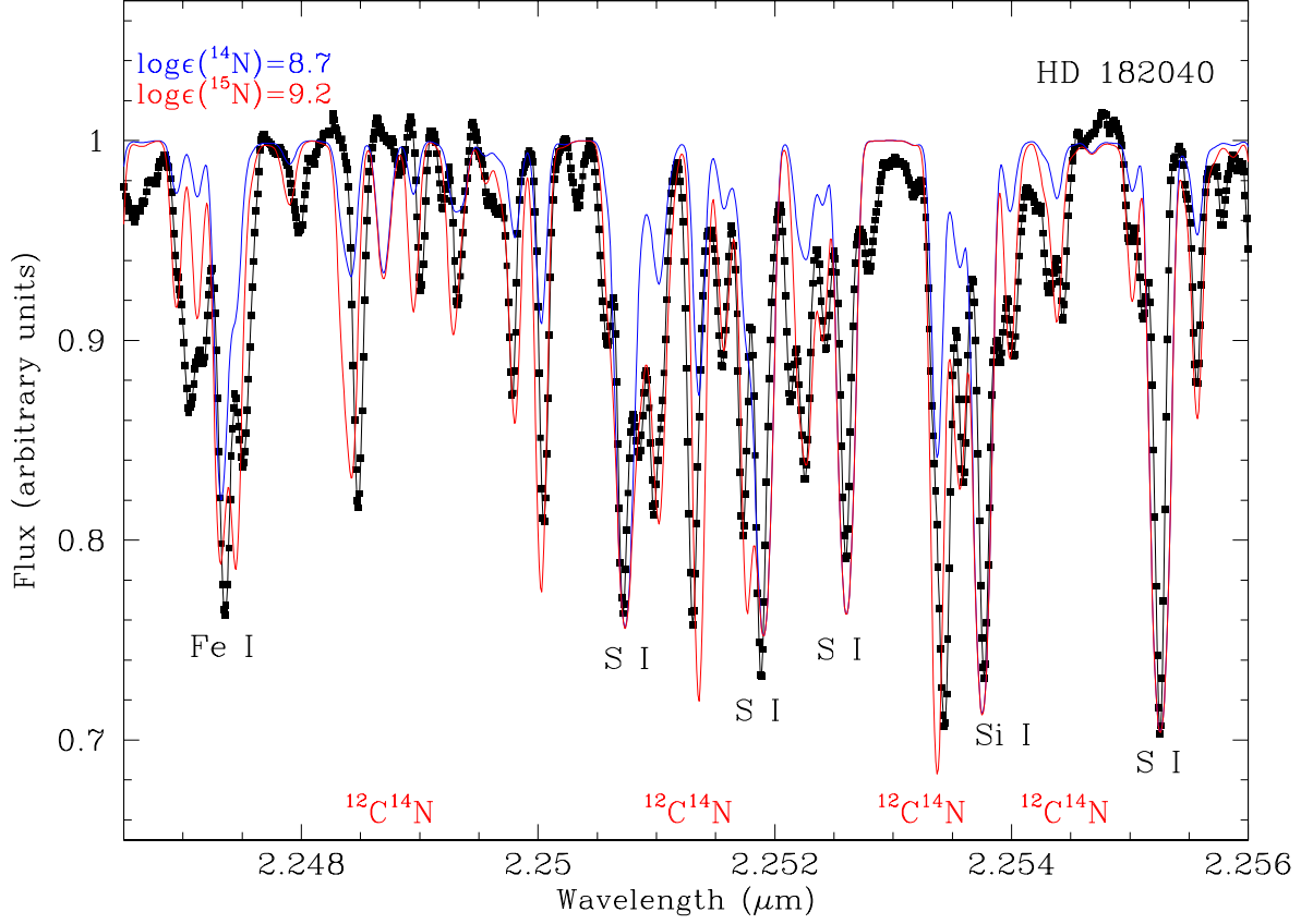
Fig. 16.— Best synthetic (red) and observed (black) spectrum for the CN region centered at \sim 2.251 \mu\text{m} for the ^{18}\text{O} -rich HdC star HD 182040. The synthetic spectrum has been created assuming the input C abundance of 9.52, the N is in the form of ^{14}\text{N} with an abundance \log \epsilon(\text{N}) = 9.2 dex, and a total O abundance of \log \epsilon(\text{O}) = 8.0 . A synthetic spectrum (blue) for a lower ^{14}\text{N} abundance of \log \epsilon(\text{N}) = 8.7 dex is also shown for comparison.
