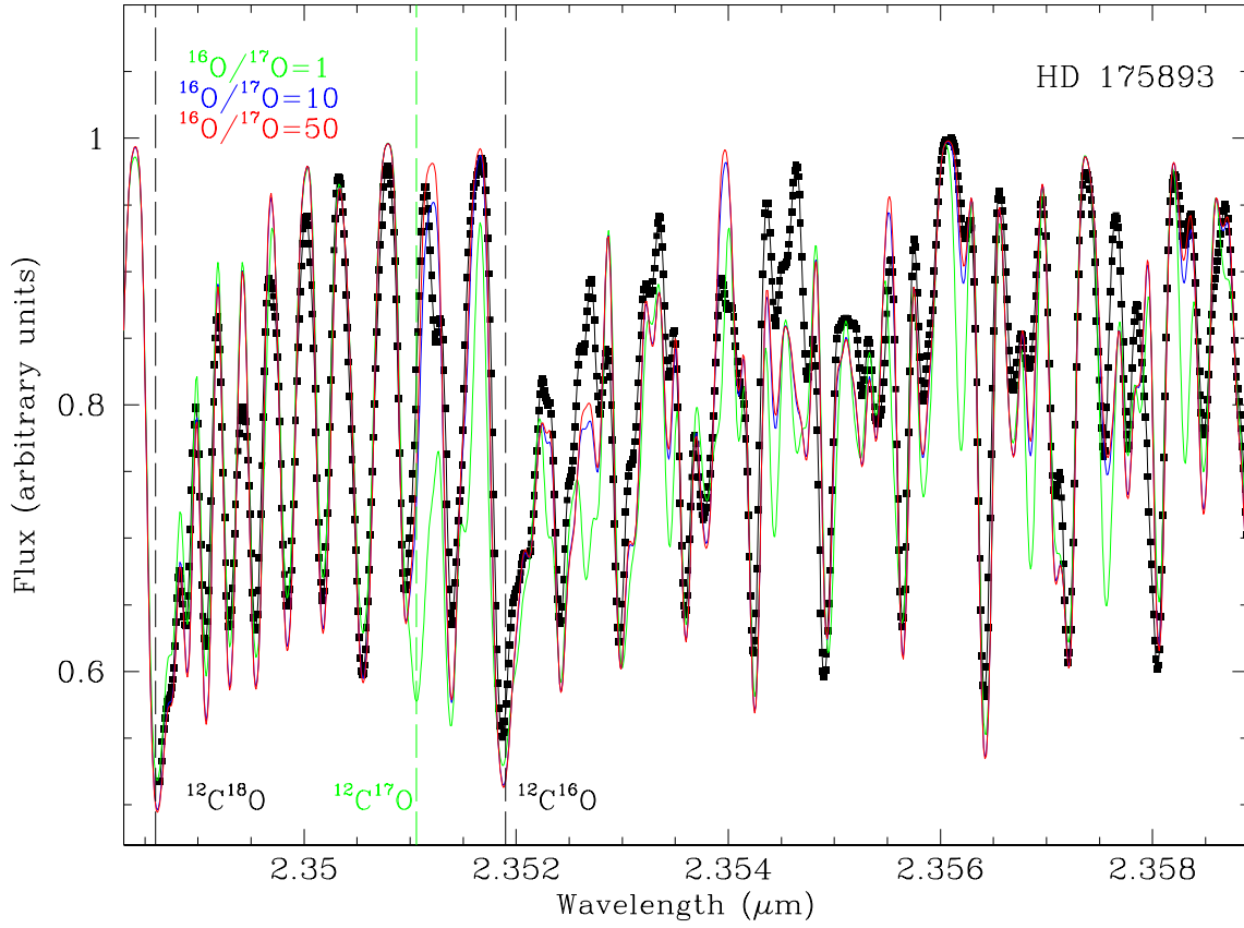
Fig. 11.— Best synthetic (red) and observed (black) spectrum in the region around the 2-0 2.349\mu\text{m} ^{12}\text{C}^{18}\text{O} bandhead for the ^{18}\text{O} -rich HdC star HD 175893. The spectrum also covers the expected position of the 3-1 2.3511\mu\text{m} ^{12}\text{C}^{17}\text{O} bandhead. The red spectrum assumes the input C abundance of 9.52, the N abundance of 9.2, a total O ( ^{16}\text{O} + ^{17}\text{O} + ^{18}\text{O} ) of \log\varepsilon(\text{O})=8.7 and the isotopic ratios ^{16}\text{O}/^{18}\text{O}=0.3 and ^{16}\text{O}/^{17}\text{O}=50 . This region contains ^{12}\text{C}^{16}\text{O} and ^{12}\text{C}^{18}\text{O} lines which are fit with the isotopic ratio ^{16}\text{O}/^{18}\text{O}=0.3 . Synthetic spectra for lower ^{16}\text{O}/^{17}\text{O} ratios (or higher ^{17}\text{O} abundances) of 1 (green) and 10 (blue) but the same total O ( ^{16}\text{O} + ^{17}\text{O} + ^{18}\text{O} ) of \log\varepsilon(\text{O})=8.7 are shown for comparison. Note the strong dependence of the 3-1 2.3511\mu\text{m} ^{12}\text{C}^{17}\text{O} bandhead (not detected in our spectra) to changes of the ^{16}\text{O}/^{17}\text{O} ratio.
