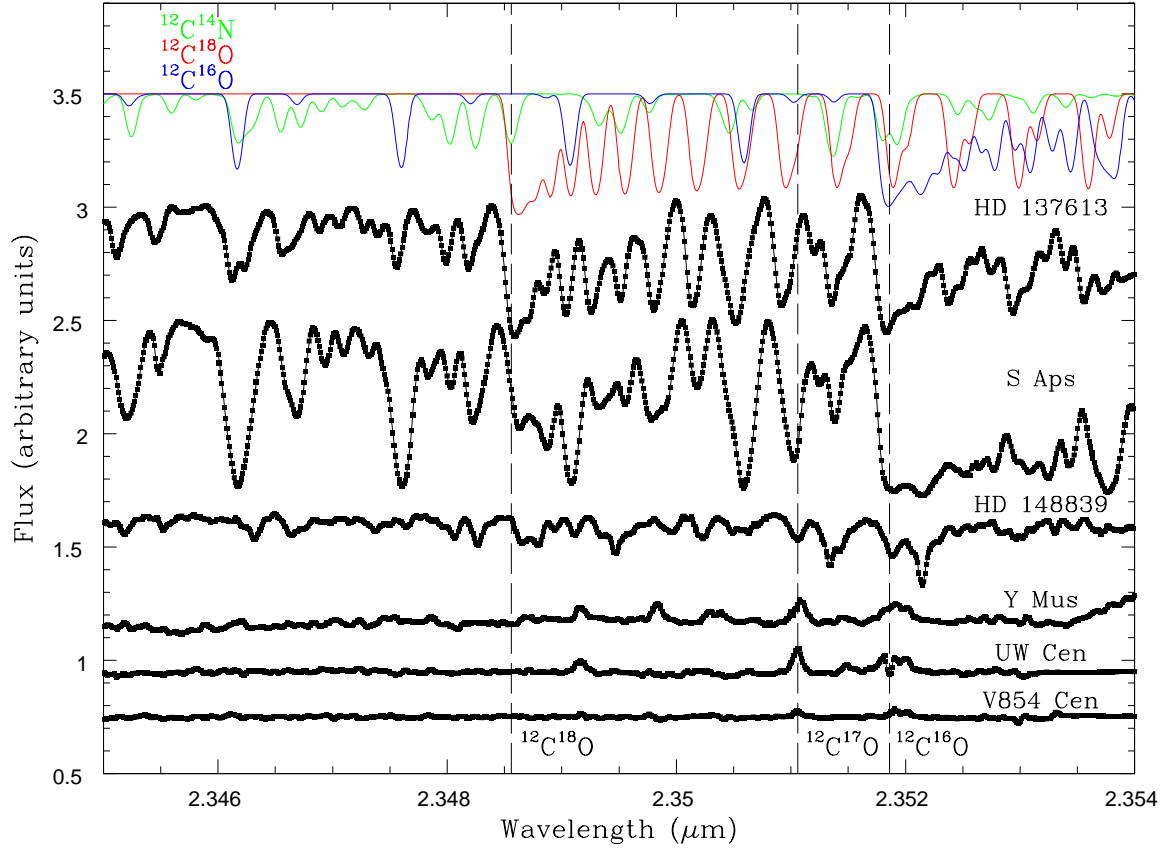
Fig. 6.— PHOENIX spectra around the 2-0 ^{12}\text{C}^{18}\text{O} at \sim 2.3485 \mu\text{m} for six stars (four RCB stars and two HdC stars): (from top to bottom) HD 137613, S Aps, HD 148839, Y Mus, UW Cen, and V854 Cen. Synthetic spectra composed for HD 137613 for the CO isomers ( ^{12}\text{C}^{16}\text{O} in blue and ^{12}\text{C}^{18}\text{O} in red) and for the ^{12}\text{C}^{14}\text{N} isomer (in green) are shown at the top for comparison. The apparent emission features in the spectra of the Y Mus, UW Cen, and V854 Cen arise from incomplete cancelling of telluric lines. See the caption of Figure 5 for additional information.
