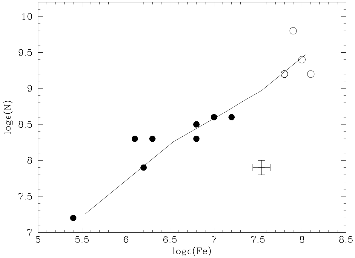
Fig. 23.— Nitrogen abundances for EHe stars (filled circles) and HdC stars (open circles) as a function of the Fe abundances. The solid line represents the N abundance being equal to the sum of the initial C, N, and O abundances expected from the Fe abundance. The solar N and Fe abundances are indicated by a large cross.
