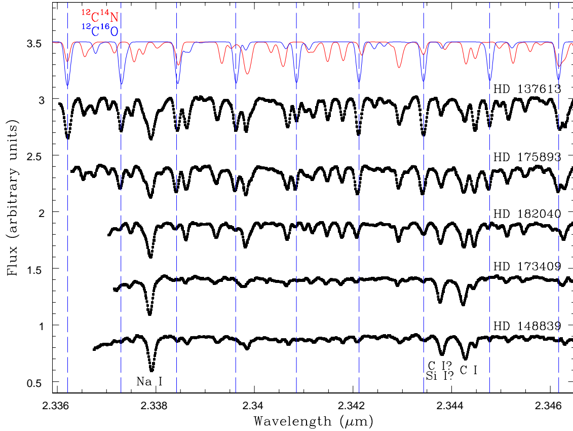
Fig. 4.— PHOENIX spectra centered at 2.341 \mu\text{m} for the five HdC stars. As for Figure 3, this region is dominated by ^{12}\text{C}^{16}\text{O} and ^{12}\text{C}^{14}\text{N} lines but note the NaI line at 2.3379 \mu\text{m} . See the caption of Figure 3 for additional information.
