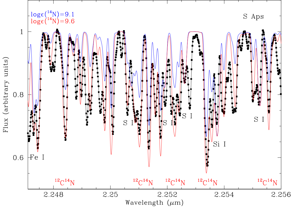
Fig. 21.— Best synthetic (red) and observed (black) spectrum for the CN region centered at \sim 2.251 \mu\text{m} for the ^{18}\text{O} -rich RCB star S Aps. The synthetic spectrum has been created assuming the input C abundance of 9.52, the N is in the form of ^{14}\text{N} with an abundance \log \varepsilon(\text{N})=9.6 dex, and a total O abundance of \log \varepsilon(\text{O})= 9.4 . A synthetic spectrum (blue) for a lower ^{14}\text{N} abundance of \log \varepsilon(\text{N})=9.1 dex is also shown for comparison.
