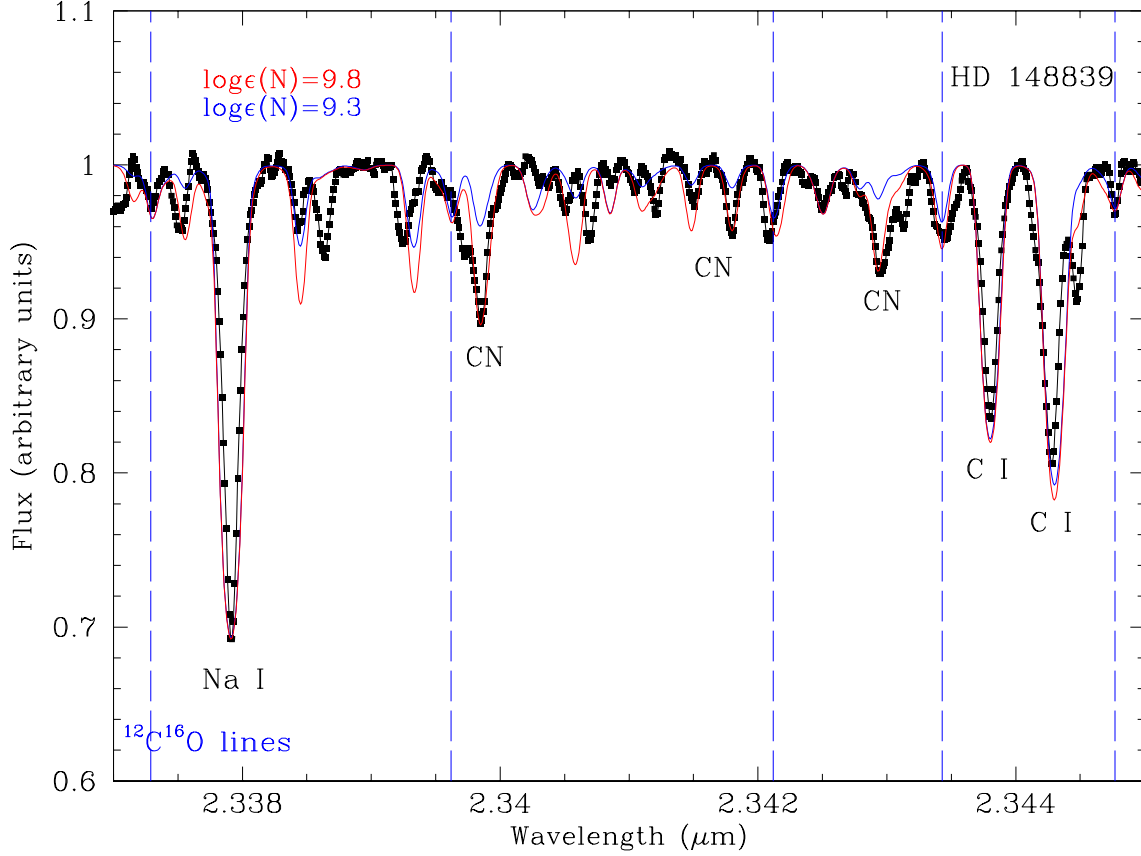
Fig. 20.— Best synthetic (red) and observed (black) spectrum for the CO and CN region centered at \sim 2.341 \mu\text{m} for the HdC star HD 148839. The synthetic spectrum has been created assuming the input C abundance of 9.52, the N is in the form of ^{14}\text{N} with an abundance \log\epsilon(\text{N})=9.8 dex, and a total O abundance of \log\epsilon(\text{O})=9.2 . A synthetic spectrum for a lower ^{14}\text{N} abundance of \log\epsilon(\text{N})=9.3 (in blue) is also shown for comparison.
