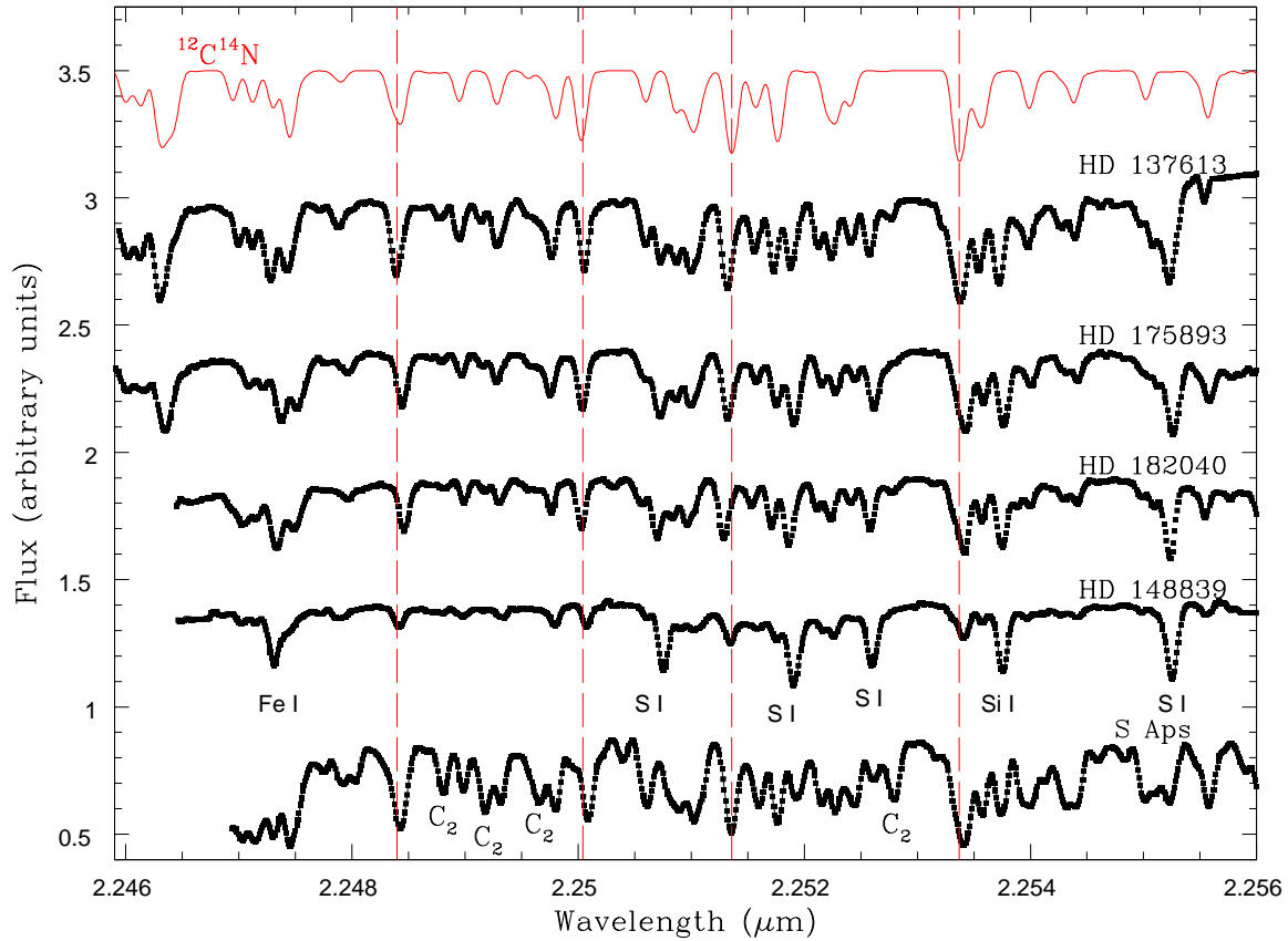
Fig. 1.— PHOENIX spectra centered at \sim 2.251 \mu\text{m} for four HdC stars (from top to bottom: HD 137613, HD 175893, HD 182040, and HD 148839, respectively). The spectrum of the RCB star S Aps is also shown. Positions of several atomic lines are labeled. The strongest ^{12}\text{C}^{14}\text{N} features are indicated with a dashed red vertical line. A ^{12}\text{C}^{14}\text{N} synthetic spectrum (in red) composed for HD 137613 is shown at the top. Phillips system \text{C}_2 lines labeled are 1-3 R22, 0-2 Q34, 1-3 Q8 and 1-3 Q10 in order of increasing wavelength.
