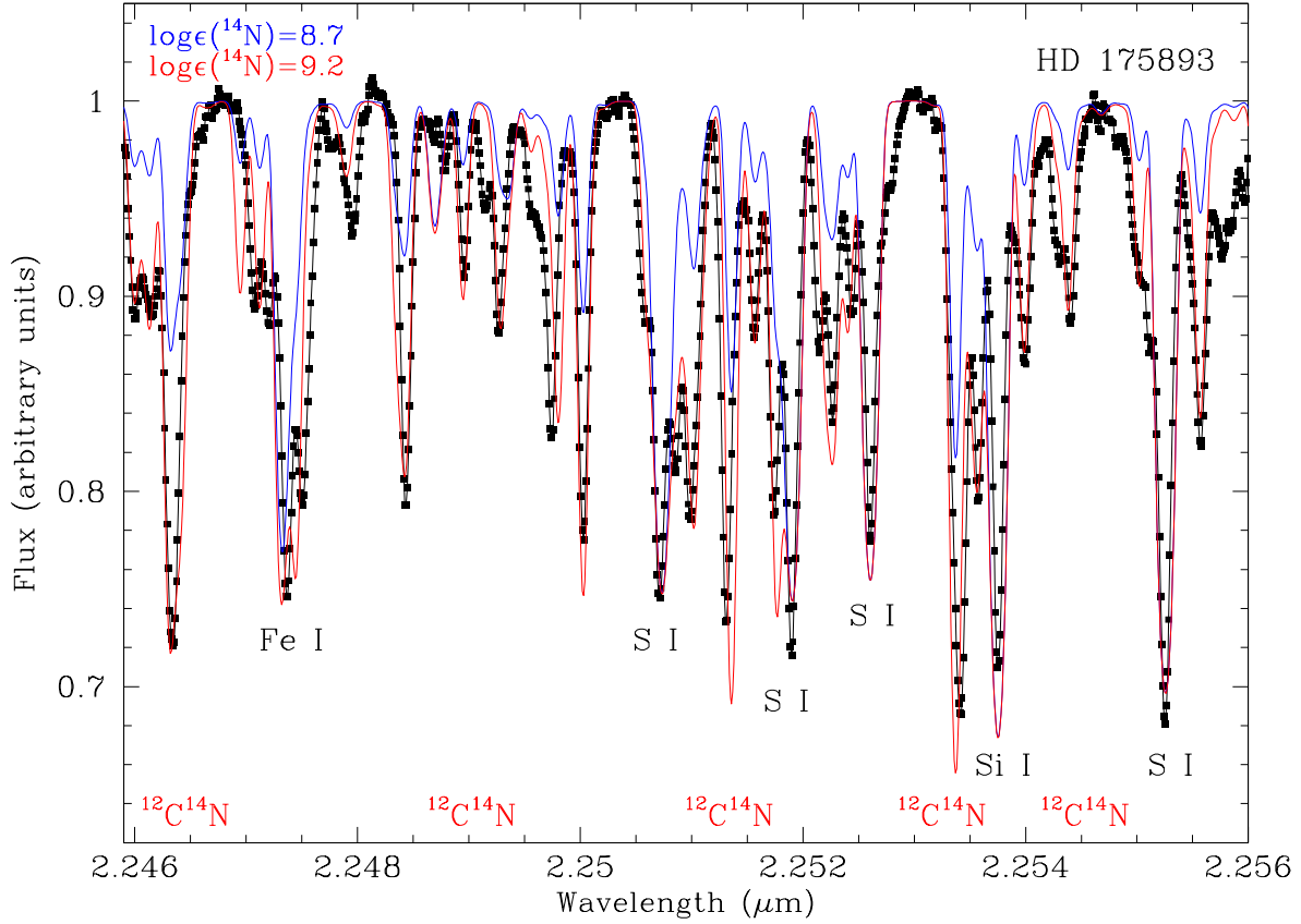
Fig. 8.— Best synthetic (red) and observed (black) spectrum for the CN region centered at \sim 2.251 \mu\text{m} for the ^{18}\text{O} -rich HdC star HD 175893. The synthetic spectrum has been created assuming the input C abundance \log \epsilon(\text{C})=9.52 , the N is in the form of ^{14}\text{N} with an abundance \log \epsilon(\text{N})=9.2 , and a total O abundance of \log \epsilon(\text{O})=8.7 . A synthetic spectrum (blue) for a lower ^{14}\text{N} abundance of \log \epsilon(\text{N})=8.7 dex is shown for comparison. Note the strong dependence of the ^{12}\text{C}^{14}\text{N} lines to changes of the elemental N abundance.
