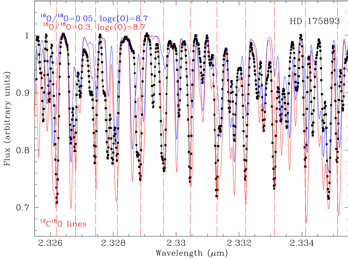
Fig. 9.— Best synthetic (red) and observed (black) spectrum for the wavelength region centered around 2.332 \mu\text{m} for the ^{18}\text{O} -rich HdC star HD 175893. The red spectrum assumes the input C abundance of 9.52, the N abundance of 9.2, a total O ( ^{16}\text{O} + ^{18}\text{O} ) of \log \epsilon(\text{O})=8.7 , and the isotopic ratio ^{16}\text{O}/^{18}\text{O}=0.3 . This region contains ^{12}\text{C}^{16}\text{O} but not ^{12}\text{C}^{18}\text{O} lines and the ^{12}\text{C}^{16}\text{O} lines are fit with the isotopic ratio ^{16}\text{O}/^{18}\text{O}=0.3 (or \log \epsilon(^{16}\text{O})=8.1 ). The synthetic spectrum also includes CN lines. A synthetic spectrum (blue) for a lower ^{16}\text{O}/^{18}\text{O} ratio of 0.05 (or a lower ^{16}\text{O} abundance) but the same total O ( ^{16}\text{O} + ^{18}\text{O} ) of \log \epsilon(\text{O})=8.7 is shown for comparison. Note the strong dependence of the most clear ^{12}\text{C}^{16}\text{O} lines (marked with red dashed vertical lines) to changes of the ^{16}\text{O} abundance.
