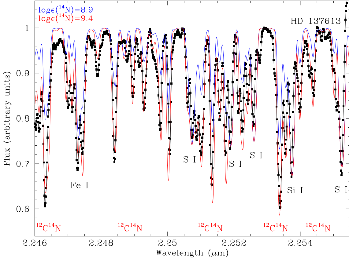
Fig. 13.— Best synthetic (red) and observed (black) spectrum for the CN region centered at \sim 2.251 \mu\text{m} for the ^{18}\text{O} -rich HdC star HD 137613. The synthetic spectrum has been created assuming the input C abundance of 9.52, the N is in the form of ^{14}\text{N} with an abundance \log\epsilon(\text{N})=9.4 dex, and a total O abundance of \log\epsilon(\text{O})=8.7 . A synthetic spectrum (blue) for a lower ^{14}\text{N} abundance of \log\epsilon(\text{N})=8.9 dex is also shown for comparison.
