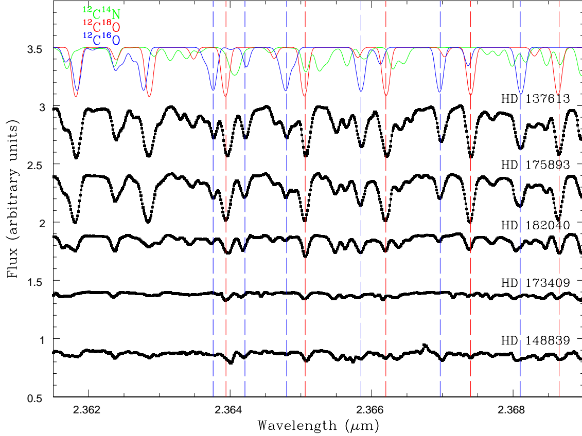
Fig. 7.— PHOENIX spectra centered at 2.365 \mu\text{m} of the five known HdC stars. Synthetic spectra composed for HD 137613 for the CO isomers ( ^{12}\text{C}^{16}\text{O} in blue and ^{12}\text{C}^{18}\text{O} in red) and for the ^{12}\text{C}^{14}\text{N} isomer (in green) are shown at the top for comparison. Note that individual isotopic molecular lines of ^{12}\text{C}^{18}\text{O} and ^{12}\text{C}^{16}\text{O} are clearly resolved and marked with dashed vertical lines.
