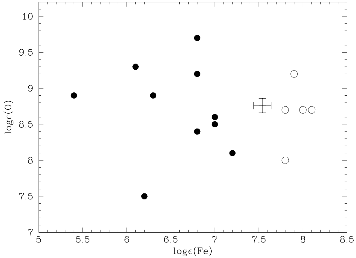
Fig. 24.— Oxygen abundances for EHe stars (filled circles) and HdC stars (open circles) as a function of the Fe abundances. As in Figure 23, the solar O and Fe abundances are indicated by a large cross.
