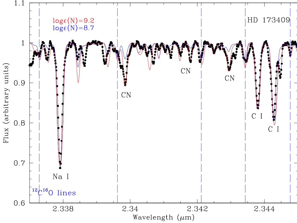
Fig. 18.— Best synthetic (red) and observed (black) spectrum for the CO and CN region centered at \sim 2.341 \mu\text{m} for the HdC star HD 173409. The synthetic spectrum has been created assuming the input C abundance of 9.52, the N is in the form of ^{14}\text{N} with an abundance \log\epsilon(\text{N})=9.2 dex, and a total O abundance fixed at \log\epsilon(\text{O})=8.7 . A synthetic spectrum for a lower ^{14}\text{N} content of \log\epsilon(\text{N})=8.7 (in blue) is also shown for comparison.
