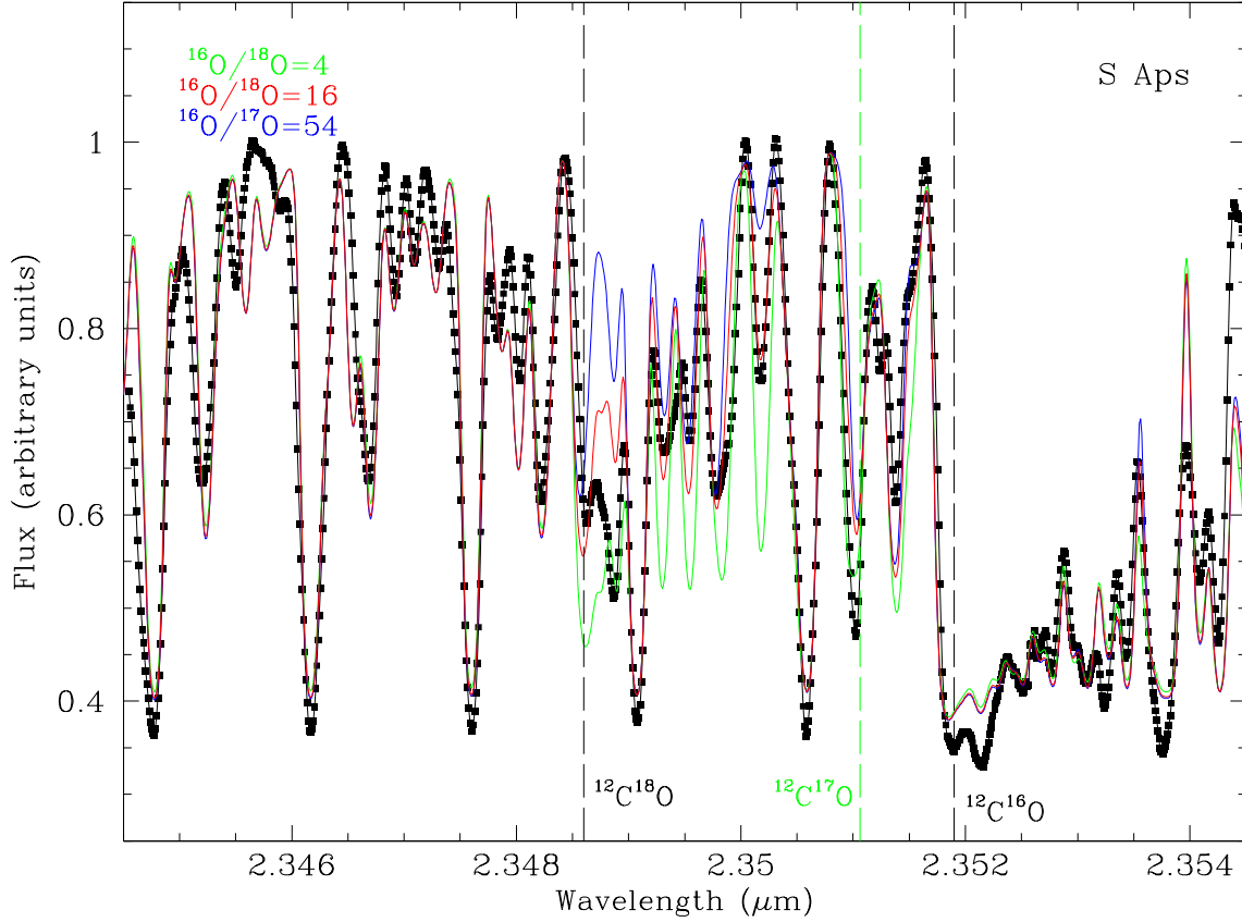
Fig. 22.— Best synthetic (red) and observed (black) spectrum in the region around the 2.0–2.349 \mu\text{m} ^{12}\text{C}^{18}\text{O} bandhead for the ^{18}\text{O} -rich RCB star S Aps. The red spectrum assumes the input C abundance of 9.52, the N abundance of 9.6, a total O ( ^{16}\text{O} + ^{18}\text{O} ) of \log \varepsilon(\text{O})=9.4 and the isotopic ratio ^{16}\text{O}/^{18}\text{O}=16 . Synthetic spectra for different ^{16}\text{O}/^{18}\text{O} ratios of 4 (green) and 54 (blue) but the same total O ( ^{16}\text{O} + ^{18}\text{O} ) of \log \varepsilon(\text{O})=9.4 are shown for comparison.
