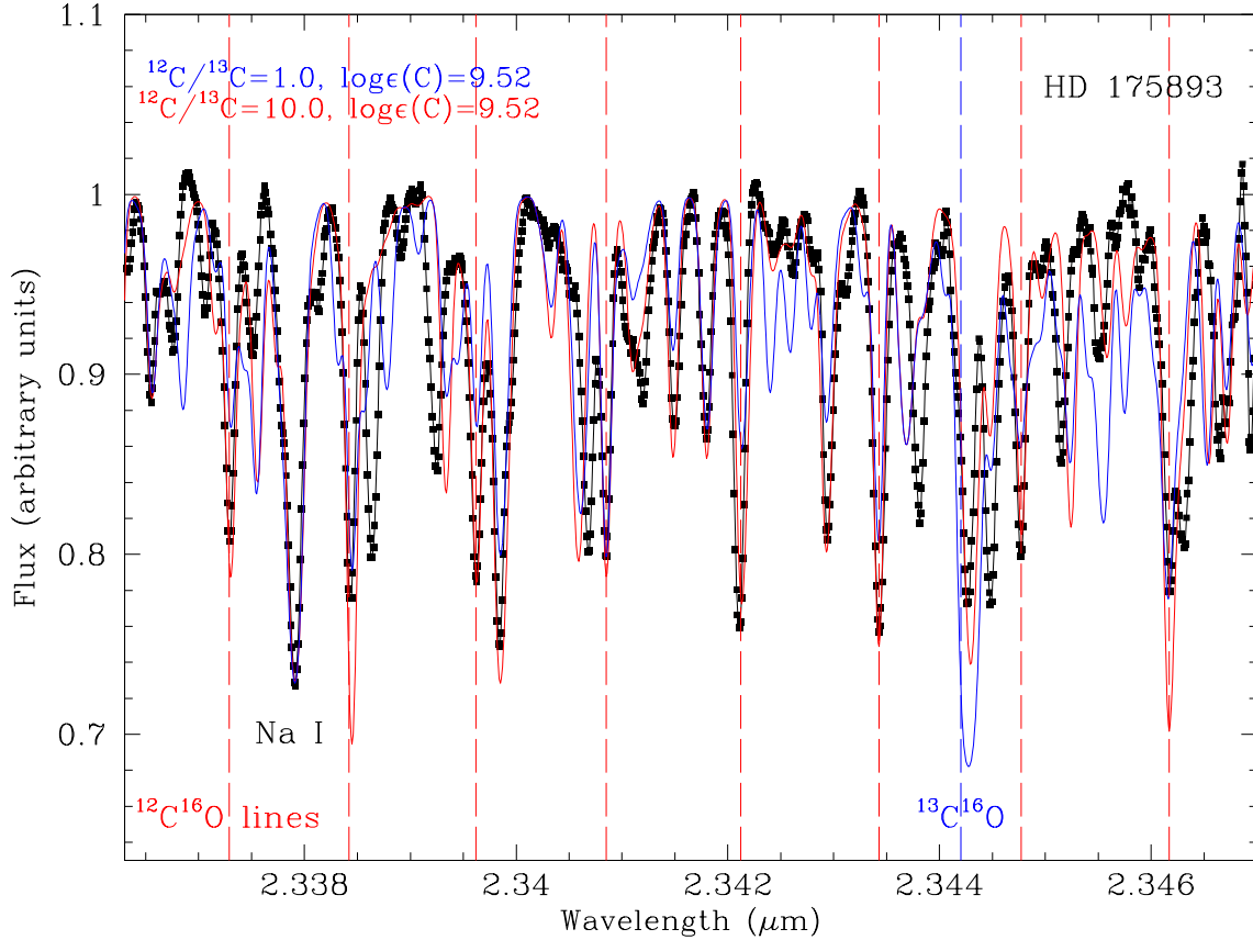
Fig. 10.— Best synthetic (red) and observed (black) spectrum in the region around the 2.344 \mu\text{m} ^{13}\text{C}^{16}\text{O} bandhead for the ^{18}\text{O} -rich HdC star HD 175893. The red spectrum assumes the input C abundance of 9.52, the N abundance of 9.2, a total O ( ^{16}\text{O} + ^{18}\text{O} ) of \log\epsilon(\text{O})=8.7 , and the isotopic ratios ^{16}\text{O}/^{18}\text{O} and ^{12}\text{C}/^{13}\text{C} of 0.3 and 10.0, respectively. This region contains ^{12}\text{C}^{16}\text{O} but not ^{12}\text{C}^{18}\text{O} lines. The 2-0 ^{13}\text{C}^{16}\text{O} bandhead is indicated with a blue dashed vertical line. The synthetic spectrum also includes CN lines. A synthetic spectrum (blue) for a lower ^{12}\text{C}/^{13}\text{C} ratio of 1.0 (or a higher ^{13}\text{C} abundance) but the same total C ( ^{12}\text{C} + ^{13}\text{C} ) of \log\epsilon(\text{C})=9.52 is shown for comparison. Note the strong dependence of the 2-0 ^{13}\text{C}^{16}\text{O} bandhead to changes of the ^{12}\text{C}/^{13}\text{C} ratio.
