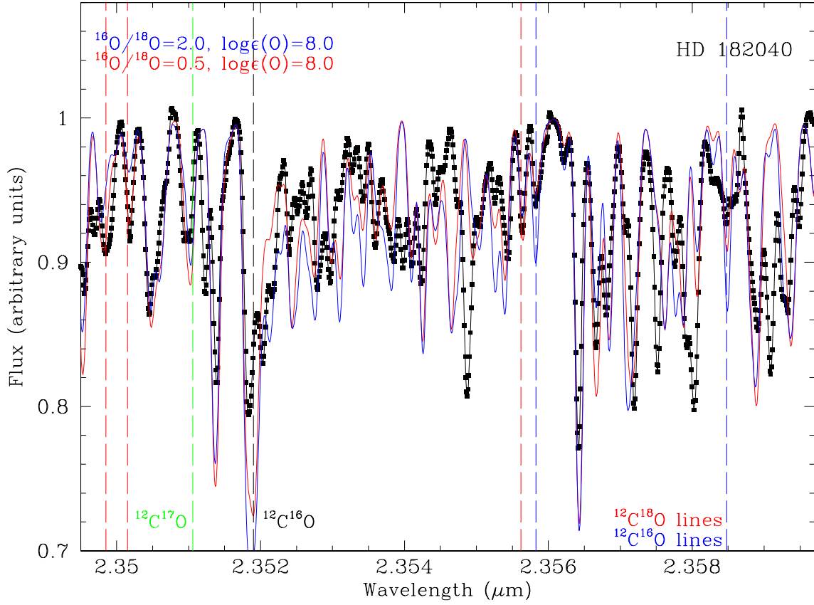
Fig. 17.— Best synthetic (red) and observed (black) spectrum in the region around the 2-0 2.349\mu\text{m} ^{12}\text{C}^{18}\text{O} bandhead for the ^{18}\text{O} -rich HdC star HD 182040. The red spectrum assumes the input C abundance of 9.52, the N abundance of 9.2, a total O ( ^{16}\text{O} + ^{18}\text{O} ) of \log\varepsilon(\text{O})=8.0 and the isotopic ratio ^{16}\text{O}/^{18}\text{O}=0.5 . A synthetic spectrum for a different ^{16}\text{O}/^{18}\text{O} ratio of 2 (blue) but the same total O ( ^{16}\text{O} + ^{18}\text{O} ) of \log\varepsilon(\text{O})=8.0 is shown for comparison. Note that there are several features (e.g. those at \sim 2.3540 , 2.3550 , 2.3575 , 2.3580 and 2.3590\mu\text{m} ) which are not reproduced by our synthetic spectra.
