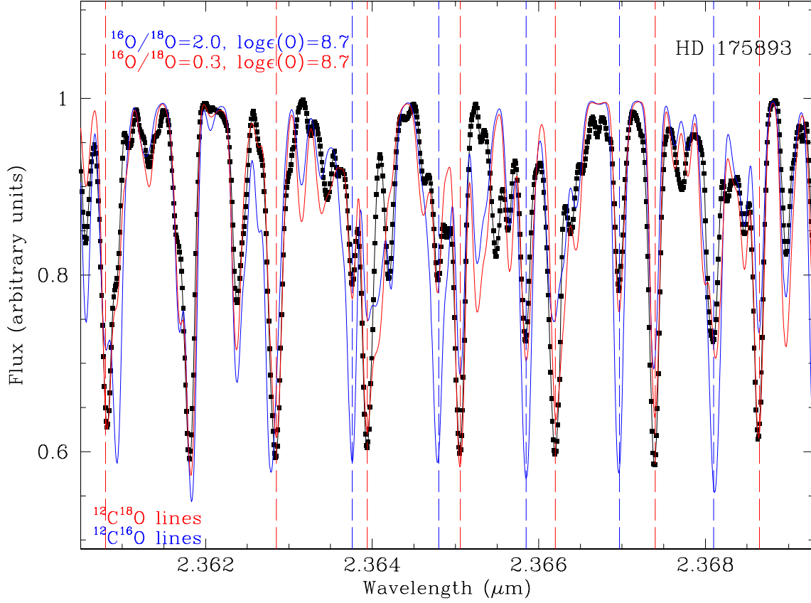
Fig. 12.— Best synthetic (red) and observed (black) spectrum for the region centered at 2.366 \mu\text{m} for the ^{18}\text{O} -rich HdC star HD 175893. The red spectrum assumes the input C abundance of 9.52, the N abundance of 9.2, a total O ( ^{16}\text{O} + ^{18}\text{O} ) of \log\epsilon(\text{O})=8.7 and the isotopic ratio ^{16}\text{O}/^{18}\text{O}=0.3 . The most clear ^{12}\text{C}^{18}\text{O} and ^{12}\text{C}^{16}\text{O} lines are marked with red and blue vertical dashed lines, respectively. A synthetic spectrum (blue) for a higher ^{16}\text{O}/^{18}\text{O} ratio of 2 (or a lower ^{18}\text{O} abundance) but the same total O ( ^{16}\text{O} + ^{18}\text{O} ) of \log\epsilon(\text{O})=8.7 is shown for comparison.
