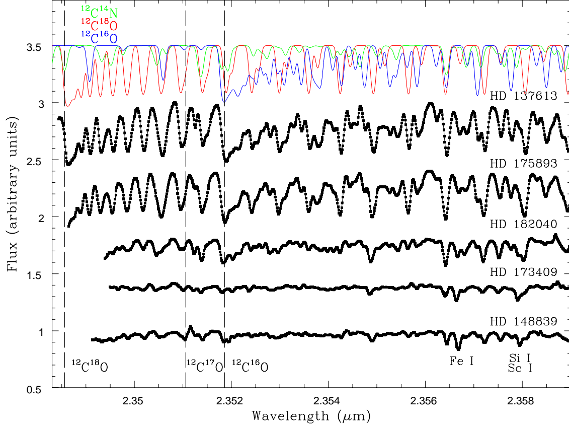
Fig. 5.— PHOENIX spectra centered at \sim 2.354 \mu\text{m} for the five known HdC stars (from top to bottom: HD 137613, HD 175893, HD 182040, HD 173409, and HD 148839, respectively). Wavelengths of 2-0 ^{12}\text{C}^{18}\text{O} , 3-1 ^{12}\text{C}^{17}\text{O} , and the 4-2 ^{12}\text{C}^{16}\text{O} bandheads are marked with a vertical dashed line. Synthetic spectra composed for HD 137613 are shown for the isomers ^{12}\text{C}^{16}\text{O} in blue, ^{12}\text{C}^{18}\text{O} in red and ^{12}\text{C}^{14}\text{N} in green.
