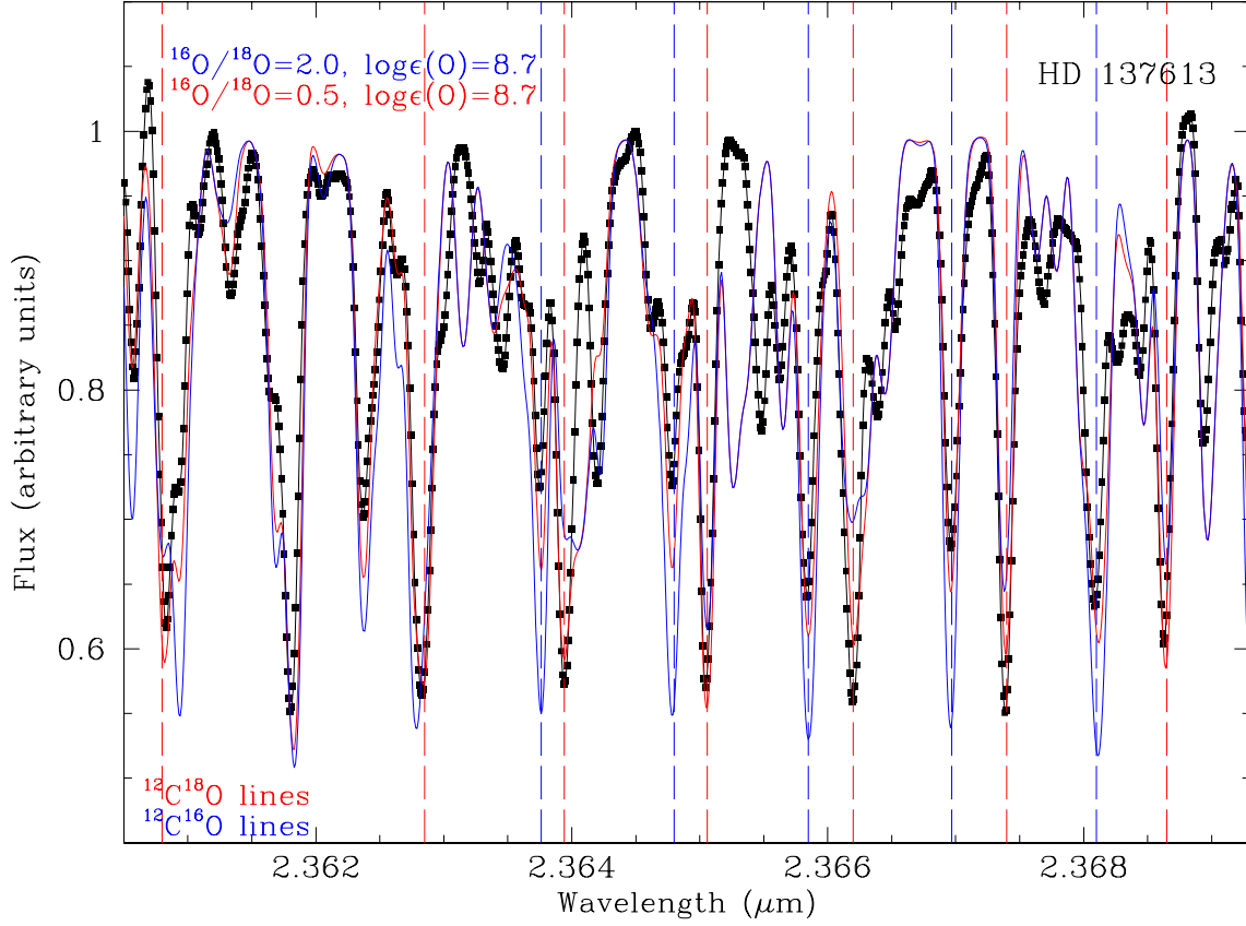
Fig. 15.— Best synthetic (red) and observed (black) spectrum for the region centered at 2.366 \mu\text{m} for the ^{18}\text{O} -rich HdC star HD 137613. The red spectrum assumes the input C abundance of 9.52, the N abundance of 9.4, a total O ( ^{16}\text{O} + ^{18}\text{O} ) of \log\epsilon(\text{O})=8.7 and the isotopic ratio ^{16}\text{O}/^{18}\text{O}=0.5 . Some of the strongest ^{12}\text{C}^{18}\text{O} and ^{12}\text{C}^{16}\text{O} lines are marked with red and blue vertical dashed lines, respectively. A synthetic spectrum (blue) for a higher ^{16}\text{O}/^{18}\text{O} ratio of 2 (or a lower ^{18}\text{O} abundance) but the same total O ( ^{16}\text{O} + ^{18}\text{O} ) of \log\epsilon(\text{O})=8.7 is shown for comparison.
