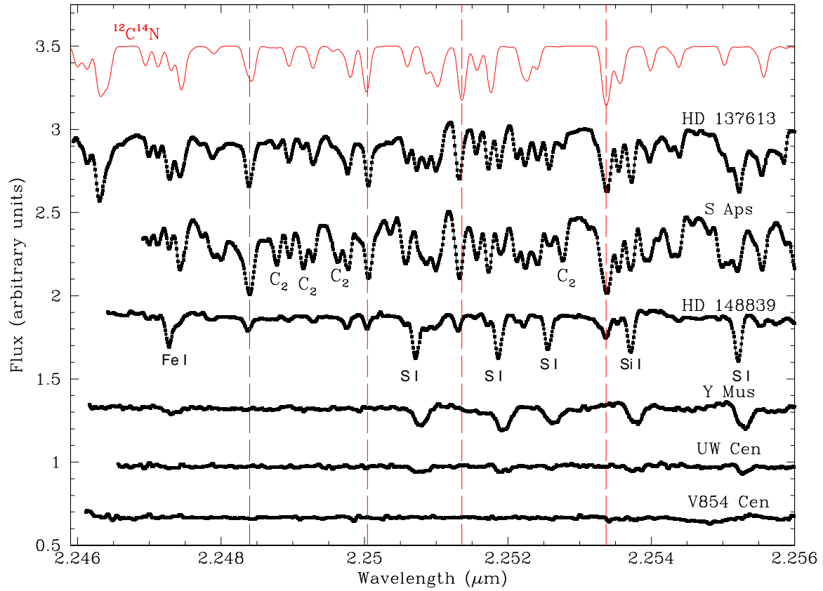
Fig. 2.— PHOENIX spectra centered at \sim 2.251 \mu\text{m} for four RCB stars and two HdC stars (from top to bottom: HD 137613, S Aps, HD 148839, Y Mus, UW Cen, and V854 Cen, respectively). See caption of Figure 1 for additional information.
