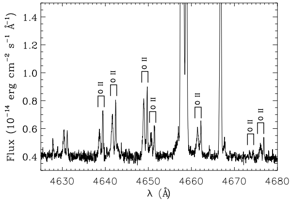
Figure 3. Section of the echelle spectrum of HH 202-S showing the shock (left) and nebular (right) components of each emission line of multiplet 1 of O II.
