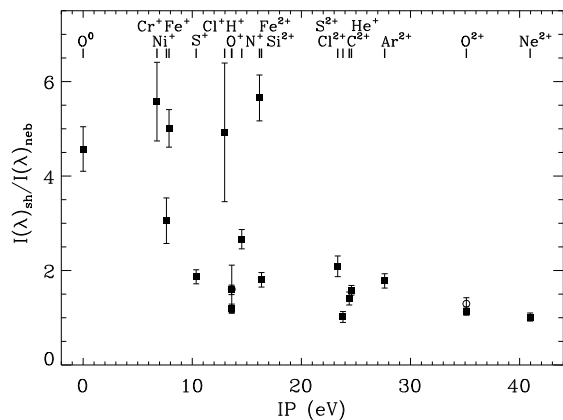
Figure 6. Weighted average of shock-to-nebular line ratios vs. the ionization potential (IP) needed to create the associated originating ion. Non-filled circles correspond to ratios measured from RLs (only for O^+ and O^{++} ). Smaller error bars are of about 3%.
