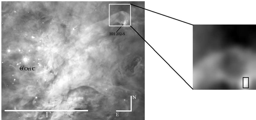
Figure 1. HST image of the central part of the Orion Nebula combined with WFPC2 images in different filters (O’Dell & Wong 1996). The white square corresponds to the field of view of the Potsdam Multi-Aperture Spectrograph (PMAS) and the separate close up image at the right shows the rebinned H\alpha map presented in Paper I. Inside of this box, the black rectangle indicates the slit position and the area covered by the UVES spectrum analyzed in this paper ( 1''5 \times 2''5 ).
