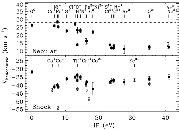
Figure 7. Heliocentric velocities of the nebular (up) and shock (down) component emission lines vs. the ionization potential (IP) needed to create the associated originating ion. The velocity of the photon dominated region (dashed horizontal line) is also shown. Non-filled triangles correspond to ions observed in only one kinematic component. Non-filled circles correspond to heliocentric velocities measured from RLs (only for O^+ and O^{++} ).
