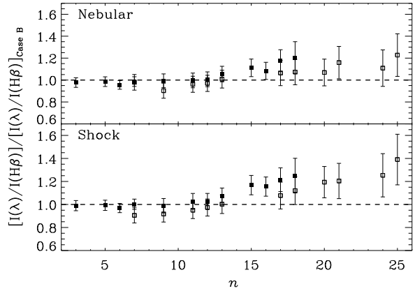
Figure 5. Dereddened fluxes of Balmer (filled squares) and Paschen (non-filled squares) lines to their theoretical flux under the Case B prediction ratio vs. the principal quantum number n for the nebular (up) and shock component (down).
