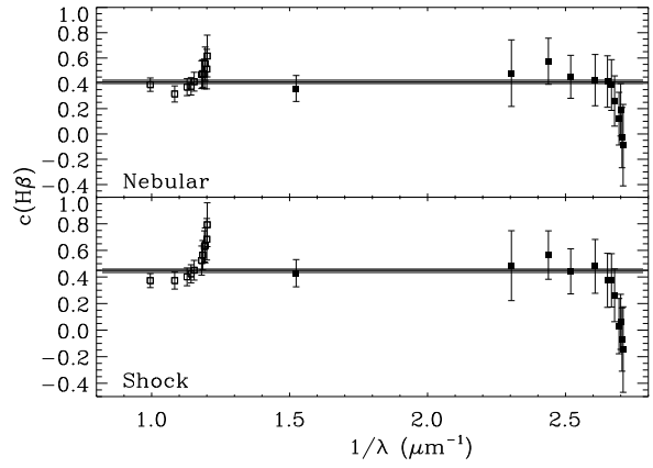
Figure 4. c(H\beta) values obtained from different line ratios vs. the inverse of the wavelength in \mu m for the nebular (up) and shock component (down). The filled and non-filled squares correspond to the c(H\beta) values derived from Balmer and Paschen lines, respectively. The horizontal line is the weighted average value adopted and the grey band its error
