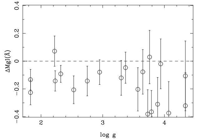
Figure 18. MgI residuals ( \Delta\text{MgI} ; observed – predicted) vs \log g for M67 stars. A significant offset of \Delta\text{MgI} = -0.134 \pm 0.022 \text{ \AA} is observed.
