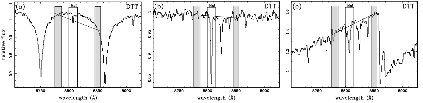
Figure 2. Index definition by DTT for the Mg I line over different spectral types. The spectra, taken from the stellar library of CEN01a, correspond to HD161817 (A2 VI; a ), HD25329 (K1 Vsb; b ) and HD148783 (M6 III; c ). Grey and open bands illustrate, respectively, the location of continuum and central bandpasses (see Table 1). Solid lines represent the local pseudo-continua computed by means of error weighted least-squares fits to all the pixels in the continuum bandpasses.
