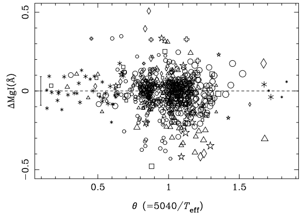
Figure 14. Residuals of the MgI fitting functions ( \Delta\text{MgI} = \text{MgI}_{\text{obs}} - \text{MgI}_{\text{pred}} ) versus \theta for the whole stellar library. See Fig. 9a for symbol codes. The error bar at the left margin indicates the unbiased residual standard deviation of the fit. See text in Sections 3.3 and 3.4 for a study on the different error sources driving the observed residuals.
