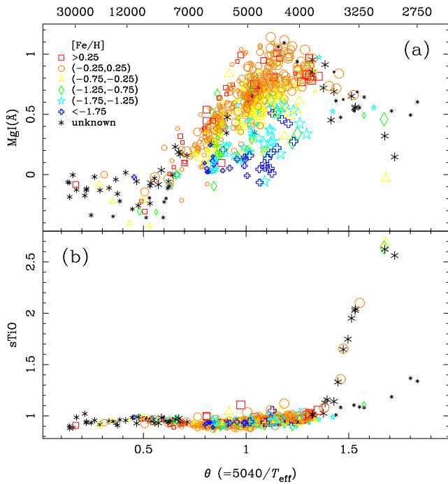
Figure 9. MgI and sTiO indices versus \theta (\equiv 5040/T_{\text{eff}}) for the whole stellar library in CEN01a. Different symbols are used to indicate different ranges of metallicities (as in the key), while sizes are related with surface gravity, in the sense that the smaller the symbol (dwarfs), the higher the gravity. On the top, the effective temperature scale is given.
