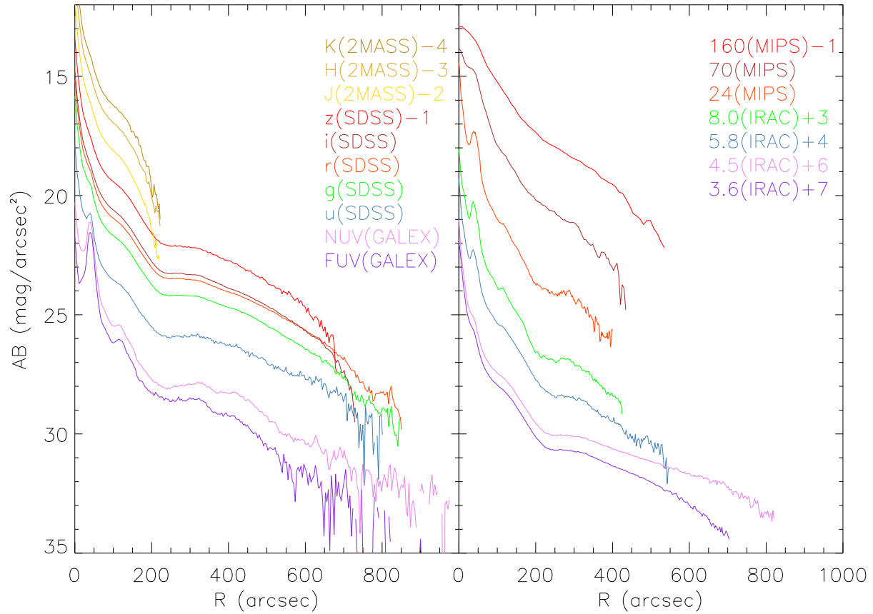
FIG. 3.— Surface brightness profiles (AB system) of M94 (NGC4736) in 17 bands ranging from the FUV to MIPS 160 \mu m.
