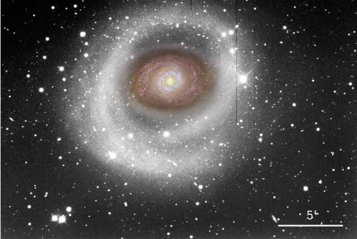
FIG. 1.— Luminance clear-filter very deep image of M94 (NGC4736) obtained with the BBRO 0.5-meter telescope. The total exposure time of the image was 555 min. The image size is 27.7' \times 18.2' . North is up and East is left. For illustrative purpose, a color image of the central part of the galaxy obtained with the same telescope has been superimposed on the inner (saturated) disk region of the galaxy. It is worth stressing that the traditional (“textbook”) picture of M94 is just what it is shown in color here.
