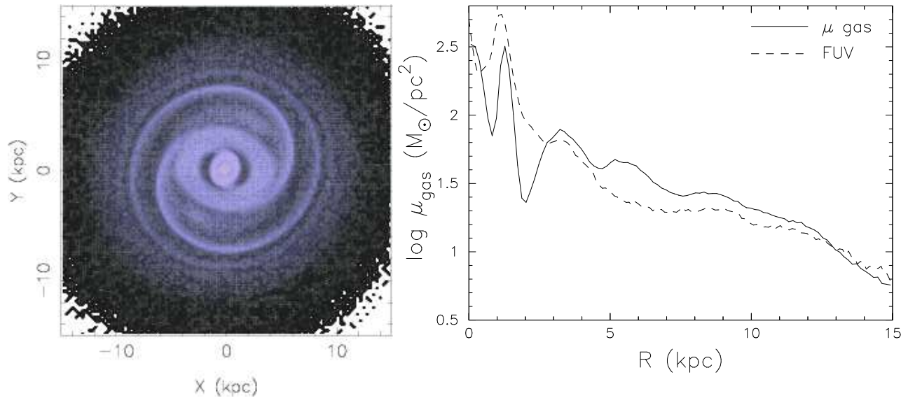
FIG. 9.— Left panel: Snapshot of the SPH simulation showing the spiral arms as a response to the inner oval distortion. On the right panel , the solid line shows the gas surface density profile of our model. The different peaks represent the response of the gas to the dynamical effect of the oval distortion. The dashed line shows the FUV surface brightness (i.e. a good proxy to the recent star formation) scaled to fit in the plot.
