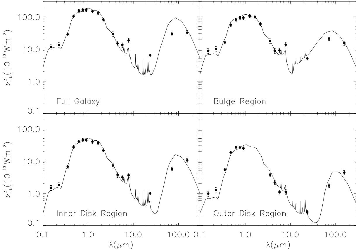
FIG. 6.— M94 (NGC4736) galaxy 0.15–160 \mu\text{m} SEDs of the total galaxy, its bulge, inner disk and outer disk regions. The solid points are the observed data and the line is the best fit model.
