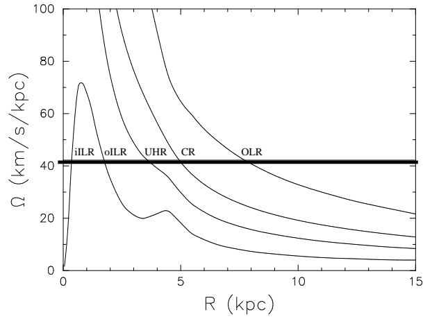
FIG. 8.— Angular frequency of the proposed model. The solid horizontal line is the pattern speed chosen in this paper.
