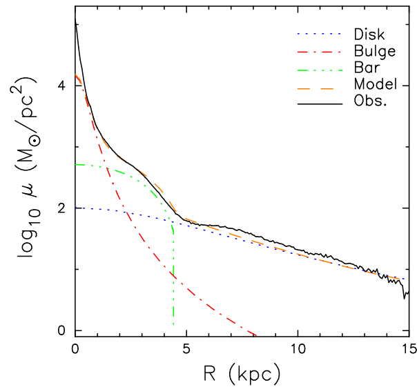
FIG. 7.— Fit to the surface density profile (shown in Fig. 4) using different analytical components. The oval distortion (inner disk) is modeled with a Ferrers bar with n=1 . The bulge, outer disk and halo are fit using Miyamoto-Nagai models.
