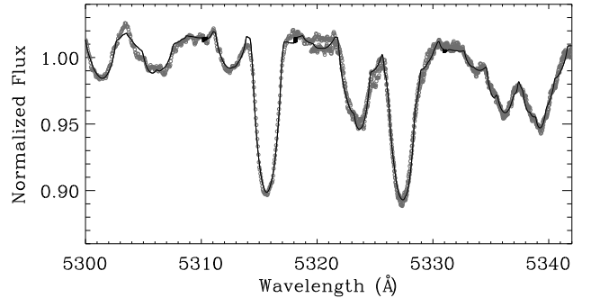
Fig. 6. The disentangled observed primary spectrum (open circles), and the theoretical fitted spectrum (solid) obtained using the abundances from Table 4.
