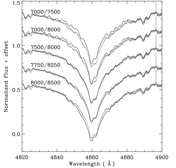
Fig. 5. Composite rotationally broadened RV- and \gamma -shifted spectral templates (black) with observations (grey) for various combinations of T_{\text{eff}} (K) for the primary and secondary components.
