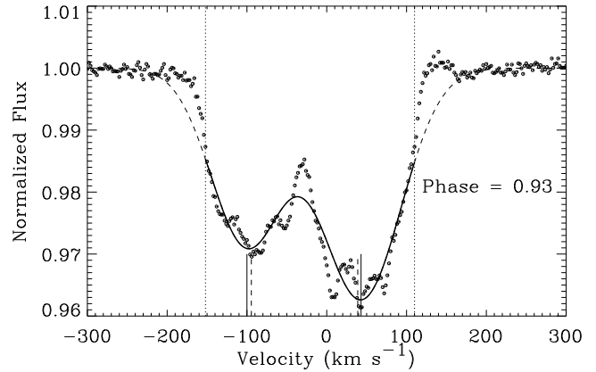
Fig. 1. Least-squares deconvolution (LSD) profile (open circles) calculated at phase 0.93 (based on T_{\min} = 2452914.644 HJD from MR05) by summing and weighting all of the lines in the spectrum. The solid curve is the double-Gaussian function fitted to the LSD profile using just the data points within the region delimited by the dotted vertical lines. We have highlighted the extracted RVs from the LSD+GAU and LSD+MM methods with vertical continuous and dashed lines, respectively.
