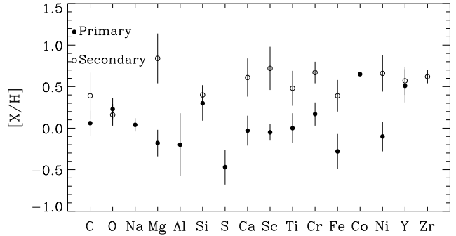
Fig. 7. Abundances of the primary (filled circles) and secondary (open circles) stars compared to the adopted solar values. The bars represent errors of \pm 1\sigma .
