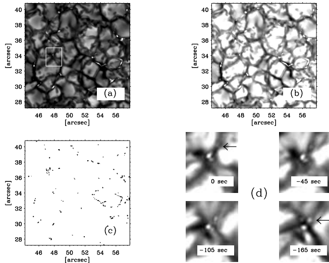
FIG. 2.— Illustration of the visual selection procedure. (a) Low contrast image of a small subfield of the FOV (see the box in Fig. 1). It is used to select the brightest G-band BPs. (b) Same image as (a) shown with high contrast. Used to identify fainter BPs. (c) Binary map with the selected structures. (d) Time series (see the insets) illustrating how an uncertain BP in the reference image (time 0 sec, the arrow) was actually a clear and conspicuous BP a few minutes before (time -165 sec, the arrow). The subfield shown in the time series is marked as a box in (a).
