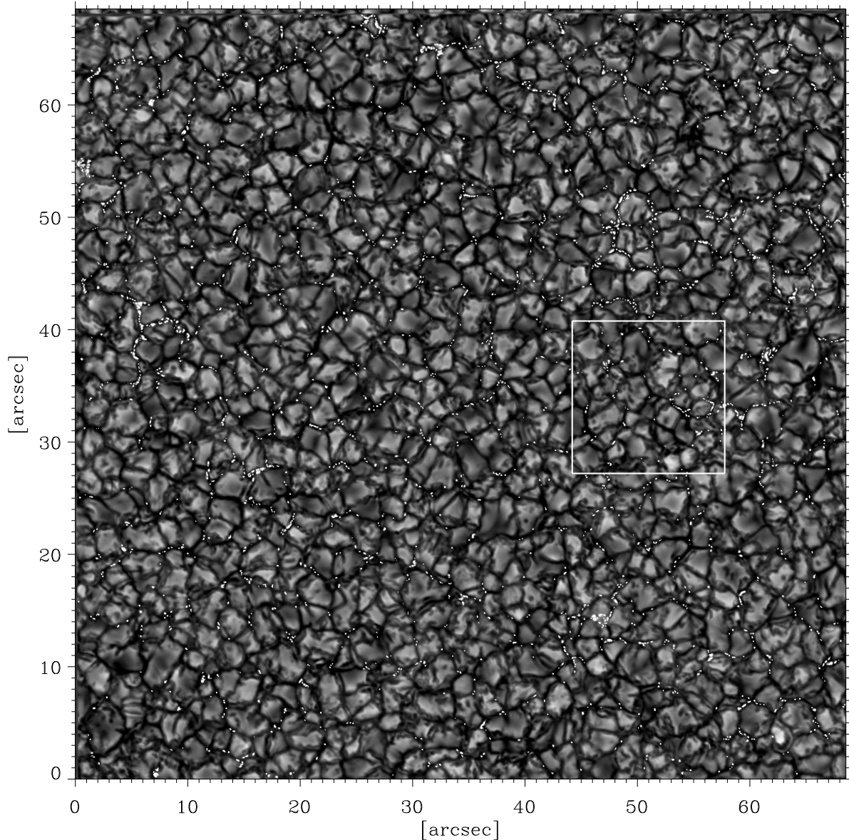
FIG. 1.— G-band image with selected BPs enhanced. BPs are found throughout, with a number density of 0.97 \text{ BPs Mm}^{-2} or, equivalently, of 1.2 \text{ BPs per granule} . The square box outlines the region blown up in Figs. 2.
