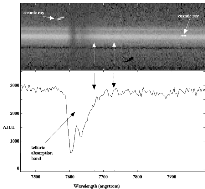
Fig. 3. Top panel: 2D spectrum of the BCG galaxy taken with the grism LR–R mounted on DOLORES in the wavelength range \sim 7500\text{--}8000\text{ \AA} . Bottom panel: 1D reduced spectrum of the BCG galaxy in the same wavelength range as above. Solid and dashed arrows indicate the position of the (hypothetical) H\alpha emission line according to the redshift given in this paper and to the redshift provided by Crawford et al. (1995), respectively. The spectrum does not show any evidence of the H\alpha emission.
