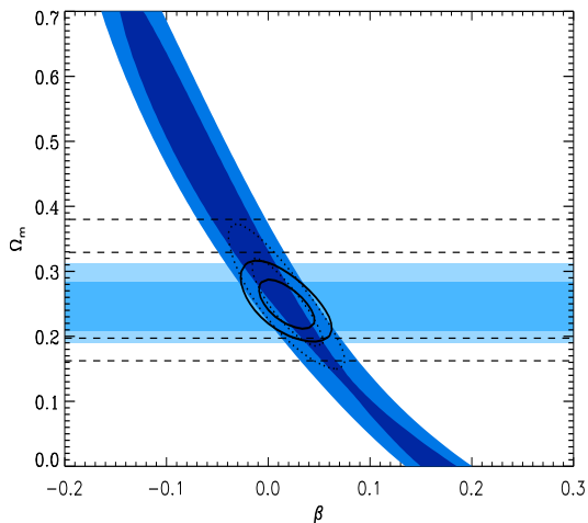
FIG. 2. Constraints from SN+ H(z) on the parameter \beta , parameterising violations of the temperature-redshift relation as T(z) = T_0(1+z)^{1-\beta} . Dark blue contours correspond to 68% and 95% confidence levels obtained from SN data alone, light blue contours are for H(z) data, and solid line transparent contours show the joint SN+ H(z) constraint. There is significant improvement from the previous constraint of reference [5] (dotted contours), which comes mainly from the inclusion of more H(z) /BAO datapoints compared to the “cosmic chronometers” determinations [45] (dashed lines) used in [5].
