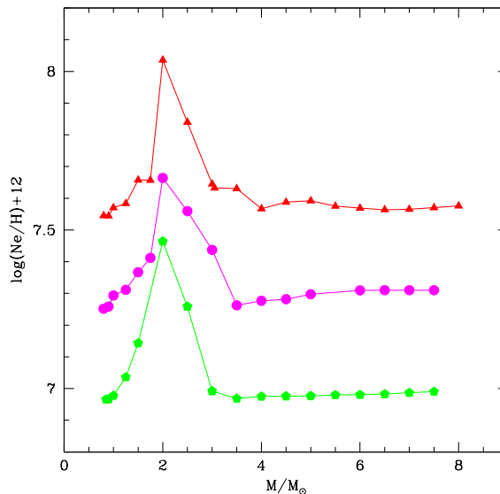
Figure 4. The final neon abundance of the models used in the present analysis as a function of the initial mass. The metallicities Z = 10^{-3} , Z = 2 \times 10^{-3} and Z = 4 \times 10^{-3} are indicated, respectively, with green pentagons, magenta circles and red triangles. The initial abundances of neon for the three cases are \log(Ne/H) + 12 = 6.93 ( Z = 10^{-3} ), \log(Ne/H) + 12 = 7.24 ( Z = 2 \times 10^{-3} ), \log(Ne/H) + 12 = 7.51 ( Z = 4 \times 10^{-3} )
