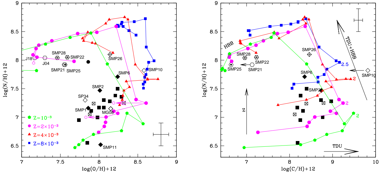
Figure 2. The observed chemical composition of the SMC PNe sample in the O-N (left panel) and C-N (right) planes. Squares, hexagons, and diamonds indicate the loci of PNe respectively of groups (a), (b) and (c) (see §5). Filled symbols mark PNe with traces of carbon dust, open-dotted symbols indicate evidence of silicates, open symbols indicate PNe with no indication of dust in the literature, and crossed symbols indicate featureless IRS spectra. We indicate the PN names for groups (b) and (c) PNe. Typical errors associated to the determination of the abundances of the individual species are indicated with crosses in the right, bottom side of the left panel and in the right, top region of the right panel. The final abundances of the AGB models of metallicity Z = 10^{-3} (green pentagons), Z = 2 \times 10^{-3} (magenta circles), Z = 4 \times 10^{-3} (red triangles), Z = 8 \times 10^{-3} (blue squares) are also shown (see legend in the O-N plot). Open, magenta circles in the left panel refer to Z = 2 \times 10^{-3} models calculated with a lower initial oxygen ( [O/Fe] = -0.2 ).
