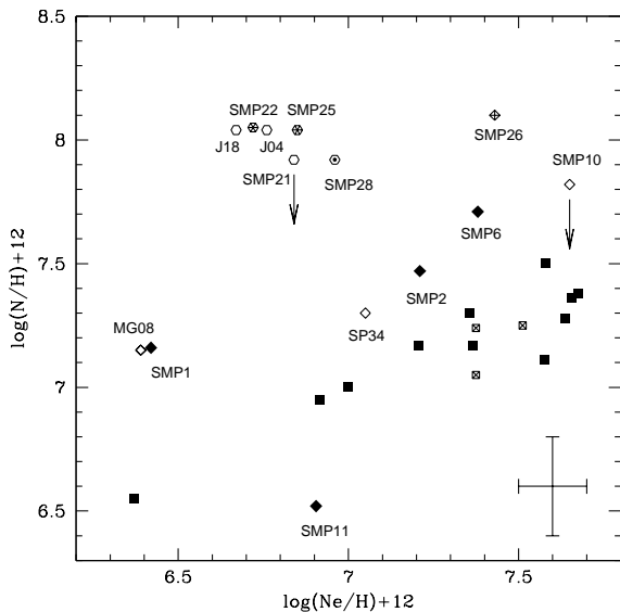
Figure 3. The nitrogen abundances of the PNe sample introduced in section 2 as a function of their neon content. The symbols are the same as in Fig. 2. The cross in the right, lower part of the plane gives the typical errors in the neon and nitrogen abundances.
