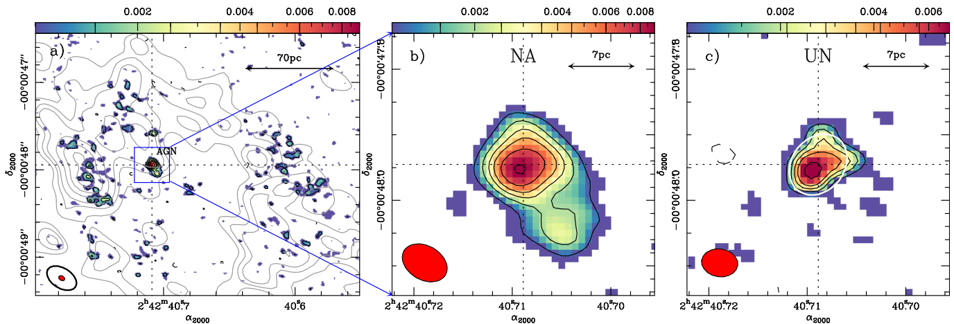
Figure 1. (a) The dust continuum emission at 694 GHz ( 432 \mu\text{m} ) mapped by ALMA in the CN of NGC 1068. The natural (NA)-weighted map is shown in color scale (in \text{Jy beam}^{-1} -units) and (black) contour levels ( 3\sigma , 5\sigma , 7\sigma , 9\sigma , 12\sigma , and 16\sigma where 1\sigma = 0.5 \text{ mJy beam}^{-1} ). The red-filled ellipse at the bottom left corner represents the beam size at 694 GHz ( 0''.07 \times 0''.05 at PA = 60^\circ ). Grey contours (10%, 20%, 30% to 90% in steps of 20% of the peak value: 49 \text{ mJy beam}^{-1} ) identify the dust emission obtained in GB14 using ALMA with a lower resolution: 0''.4 \times 0''.2 at PA = 50^\circ (black ellipse). The dashed lines highlight the location of the AGN at (\alpha_{2000}, \delta_{2000}) = (02^{\text{h}}42^{\text{m}}40.709^{\text{s}}, -00^{\circ}00'47.95'') . (b) A close-up of the dust continuum emission shown in left panel. (c) Same as middle panel but using a uniform (UN)-weighted set of data with a spatial resolution: 0''.06 \times 0''.04 at PA = 82^\circ . Contour levels are 3\sigma , 4\sigma , 5\sigma , 6\sigma , and 8\sigma where 1\sigma = 0.7 \text{ mJy beam}^{-1} . The white ellipse identifies the disk solution found by the task UV_FIT.
