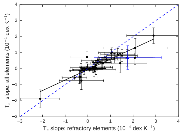
Fig. 5. T_c slopes derived by using all the elements against T_c slopes derived by considering only elements that have T_c > 900 K. The black solid line is the linear fit of the data and the blue dashed line represents the one-to-one line. The symbols are the same as in Fig. 1 and the previous plots.
