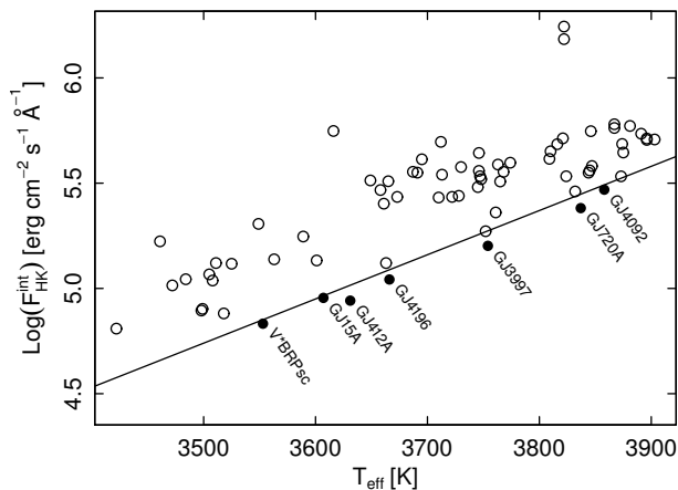
Fig. 2. F_{HK}^{int} vs. T_{eff} diagram. The solid line (Eq. 1) represent our selection threshold of reference stars. The selected stars are indicated as plain dots and their names are shown.
