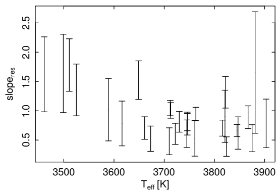
Fig. 11. Slope of the F_{\text{CaIIHK}} vs. F_{H\alpha} relationship as a function of T_{\text{eff}} . Only the stars with significant correlation ( p -value < 0.01 ) have been taken into account.
