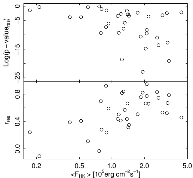
Fig. 13. p-values (top panel) and Pearson's correlation coefficient (bottom panel) of the best-fits between H\alpha and Ca II H&K fluxes shown in Fig. 7 vs. the average level of activity \langle F_{HK} \rangle .
