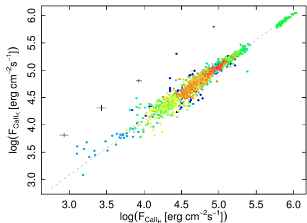
Fig. 5. \log(F_{\text{CaII}_H}) vs. \log(F_{\text{CaII}_K}) . Different colors represent different stars. The gray dashes show the RMA best fit in Eq. 2. Black crosses represent the typical measurement uncertainties at different activity levels.
