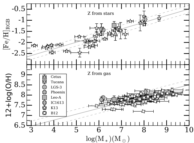
Fig. 2. Mass-metallicity relation from spectroscopy of individual stars (upper panel) and from gas-phase metallicities (lower panel) compared with the results from the LCID dwarfs. The gray line shows the fit obtained by Kirby et al. (2013) (upper panel) and Berg et al. (2012) (lower panel) in each case. For the LCID dwarfs, the [\text{Fe}/\text{H}] values have been converted into \log(\text{O}/\text{H}) + 12 using a solar scale.
