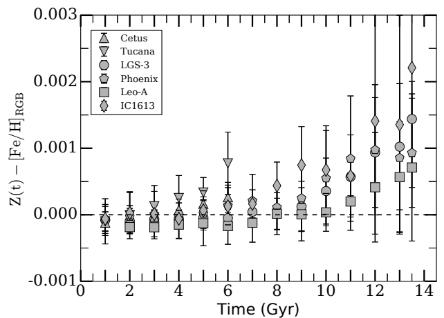
Fig. 1. Difference between Z(t) and [\text{Fe}/\text{H}]_{\text{RGB}} as a function of time for the LCID sample. The horizontal dashed line shows Z(t) = [\text{Fe}/\text{H}]_{\text{RGB}} .
