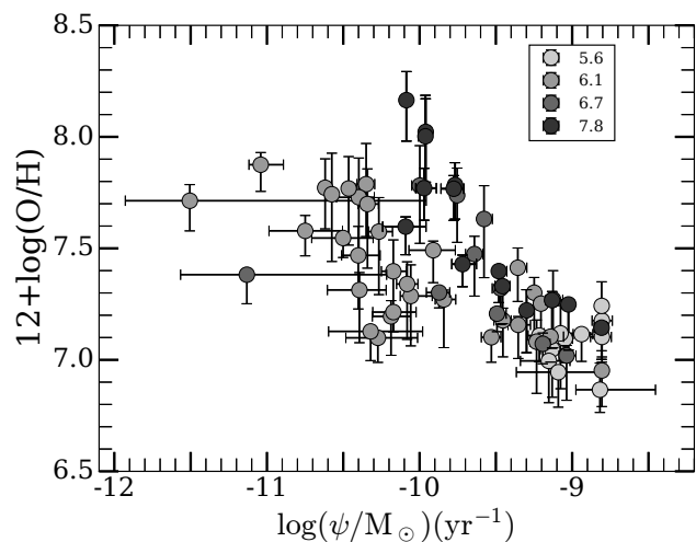
Fig. 5. Metallicity as a function of the specific SFR. The colors represent different ranges of stellar masses.
