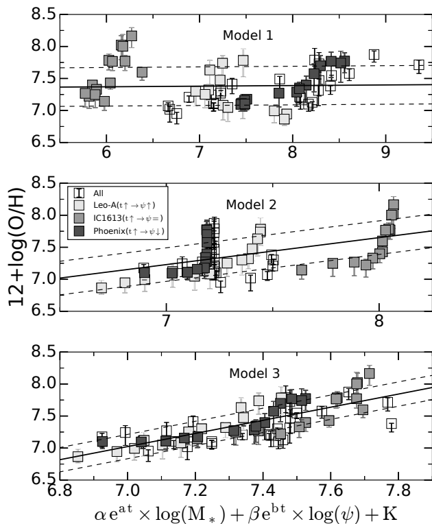
Fig. 6. Projection of Z = \alpha e^{at} \times \log(M_*) + \beta e^{bt} \times \log(\psi) for models 1 to 3 shown in Table 3. Dashed lines show the uncertainties of the fit in each case. Three galaxies are highlighted, showing three different evolutions of \psi with time: Leo-A, IC1613, and Phoenix (see text).
