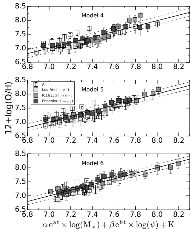
Fig. 7. Same as in Fig. 6, but for models 4 to 6.
