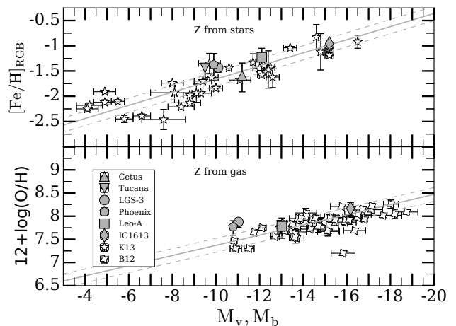
Fig. 3. Luminosity-metallicity relation obtained from the LCID dwarfs compared with the results from Kirby et al. (2013) (upper panel) and Berg et al. (2012) (lower panel). Only LCID dwarfs with non-negligible gas content are shown.
