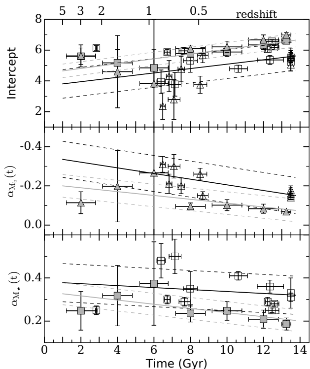
Fig. 4. Intercept (upper panel), slope of the luminosity-metallicity (middle panel), and slope of the mass-metallicity relation (lower panel) as a function of time. The open symbols show results using gas-phase metallicities from literature. The filled symbols show data from LCID dwarfs. The data obtained from M_B magnitudes are shown as triangles. The squares show results from stellar masses. The linear fits to the results are overplotted. The dashed lines show the uncertainties of the fit in each case. The vertical axis of the middle panel has been inverted to represent the same behavior as the others panels.
