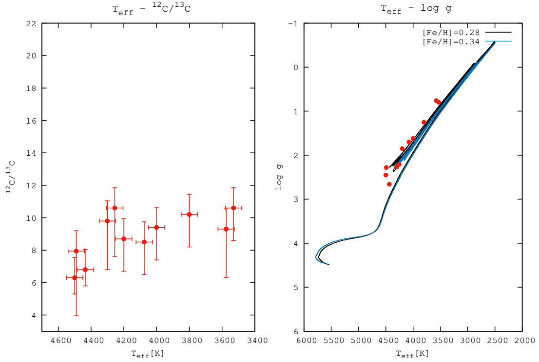
Figure 2. Left panel: ^{12}\text{C}/^{13}\text{C} ratio as a function of effective temperature from this paper. Right panel: Log g as a function of effective temperature with evolutionary tracks from Lagarde et al. (2017) at different metallicities.
