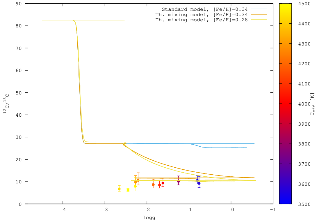
Figure 3. The evolution of the theoretical surface carbon isotopic ratio computed with STAREVOL following the standard prescription for 1.15M_{\odot} model at [\text{Fe}/\text{H}] = 0.34 (blue solid line), and including the effects of thermohaline instability for 1.1M_{\odot} model at [\text{Fe}/\text{H}] = 0.34 (orange solid line) and for 1.10M_{\odot} model at [\text{Fe}/\text{H}] = 0.28 (yellow solid line). Observations are compared with models and color-coded according to the effective temperature.
