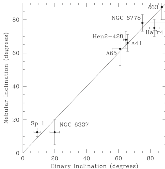
Figure 2: The observed correlation between binary and nebular inclinations in post-CE PNe, reproduced from [12].
