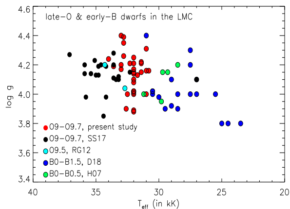
Fig. 8. T_{\text{eff}} - \log g diagram of our sample stars compared to results in the LMC for early B-type dwarfs from H07 (Hunter et al. 2007) and D18 (Dufton et al. 2018) and for late O-type dwarfs from RG12 (Rivero González et al. 2012) and SS17 (Sabín-Sanjulián et al. 2017).
