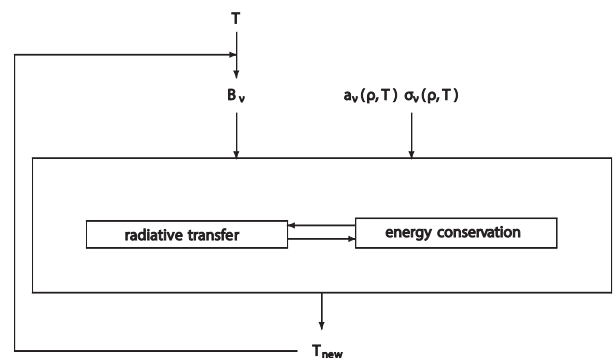
Fig. 3. The energy macro-block: simultaneous solution of the RT and RE equations. The coupling between radiative transfer and t energy conservation constraint is brought about by the scattering-like integral J_a defined by Equation (18).
