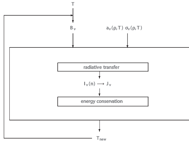
Fig. 2. Sequential solution of the energy macro-block. The transport coefficients a_\nu and \sigma_\nu are input data defined outside the block. The input temperature, initially the trial input T_0 , is the updated temperature T = T_{new} , the solution of the transcendental equation (14) at each iterative step. In the particular case here under consideration, it holds that S_\nu = B_\nu and \sigma_\nu = 0 .
