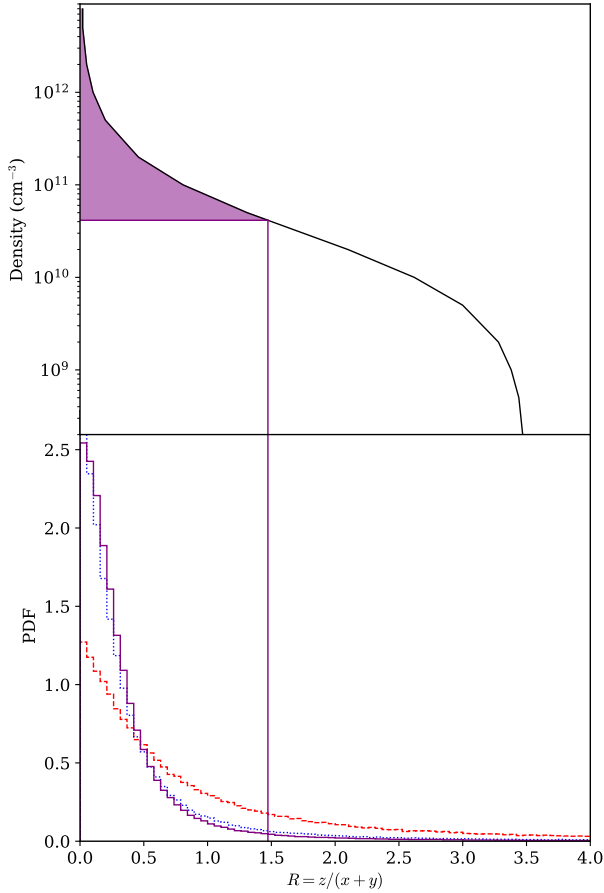
Figure 5. Constraint on density from the O VII triplet. Bottom panel: probability density of the forbidden ( z ) to intercombination ( x + y ) ratio; the vertical line marks the 95% upper limit. (Obs 2 is shown in red dashed; Obs 7 in blue dotted; and the combined observation in purple). Top panel: relation between line ratio and density, showing the corresponding lower limit to the density.
