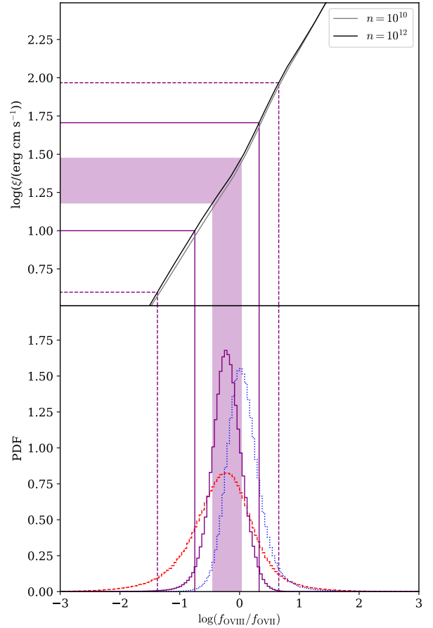
Figure 6. Constraint on the ionisation parameter from the O VIII to O VII ratio. Bottom panel: probability density of the line flux ratio (Obs 2 is shown in red dashed; Obs 7 in blue dotted; and the combined observation in purple); the shaded regions and vertical lines mark 1\sigma (68%) and 2\sigma (90%) credible intervals respectively for the combined observation. Top panel: relation between line ratio and ionisation parameter, showing the corresponding constraints on the ionisation. The black and grey lines show plasma densities of n = 10^{10} and n = 10^{12} \text{ cm}^{-3} respectively; this has only a very small effect.
