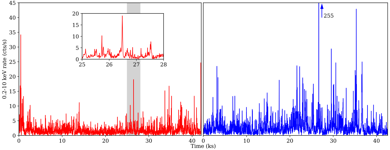
Figure 1. XMM-Newton -pn lightcurve of Swift J1858.6–0814. Observations 0831791201 and 0831791701 are shown in red and blue respectively; they are separated by around 20 days. The inset shows a zoom of the region marked in grey. The flare marked with the arrow reaches 255 cts/s. The frequent, rapid flaring displayed in these observations is typical of Swift J1858.6–0814.
