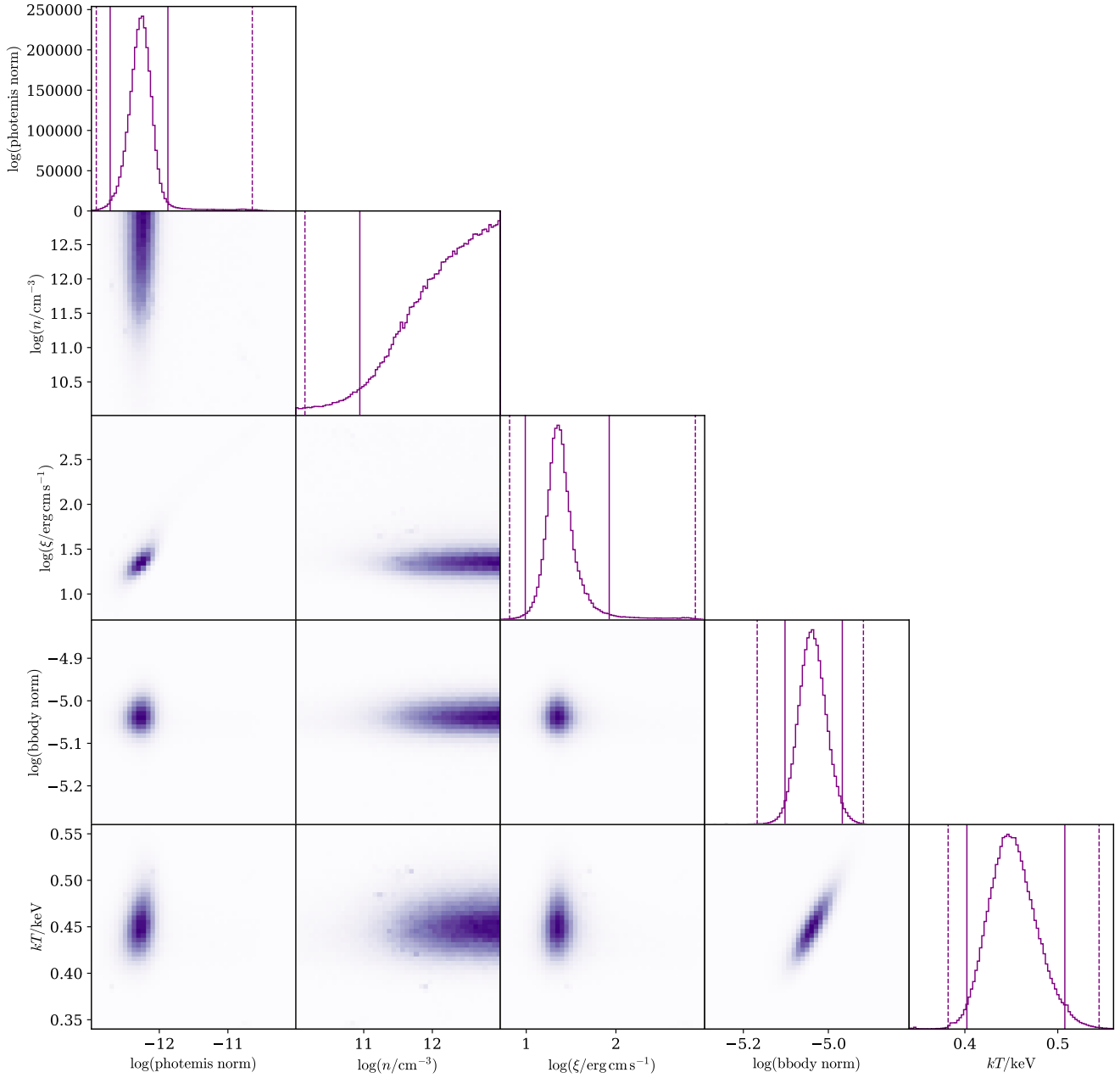
Figure 7. Posterior density plots from photoionisation modelling. Normalisations are the XSPEC values. Shaded regions, solid and dashed lines denote 68, 95 and 99.7% HPD credible regions respectively.
