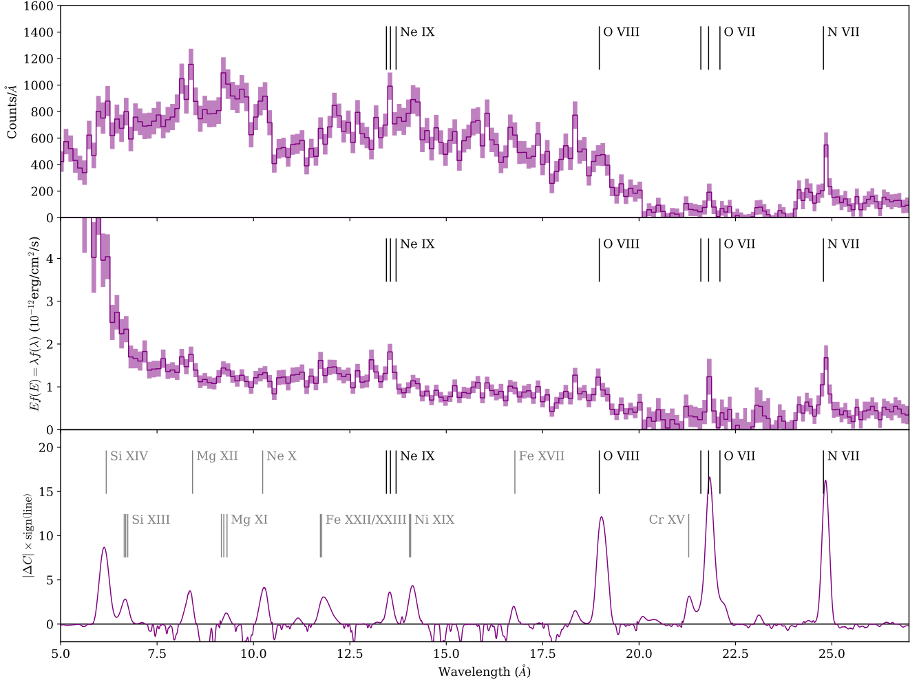
Figure 3. Combined RGS spectrum of Swift J1858.6–0814 (rebinned for plotting). Top: Background subtracted spectrum of both observations combined, shown as detected counts summed over all detectors and orders. Second row: unfolded to a \Gamma = 2 power law to remove the effect of the detector effective area. Bottom row: improvement in fit statistic from adding a narrow Gaussian to a continuum model. The magnitude gives \Delta C and the sign shows the nature of the additional line: positive represents additional emission; negative represents absorption. O VII and N VII are clearly detected; given these, O VIII is detected at the expected wavelength. Plausible transitions (grey) exist for all features with \Delta C > 4 .
