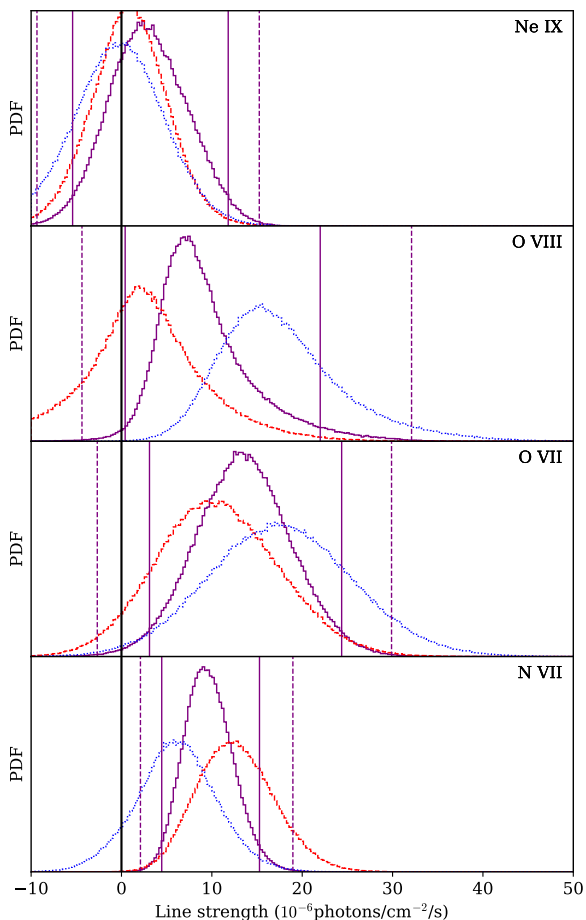
Figure 4. Posterior distributions of emission line strengths. For He-like triplets, the sum of all components is shown. Obs 2 is shown in red dashed; Obs 7 in blue dotted; and the combined observation in purple. Shaded regions, solid and dashed lines denote 68, 95 and 99.7% HPD credible regions respectively.
